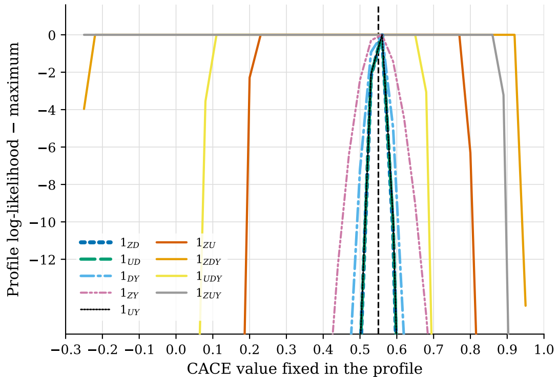
(b) Identifiable: sharp peak; nonidentifiable: flat ridge
