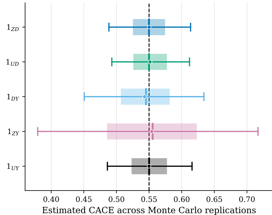
(a) Estimated CACEs center at the true CACE
