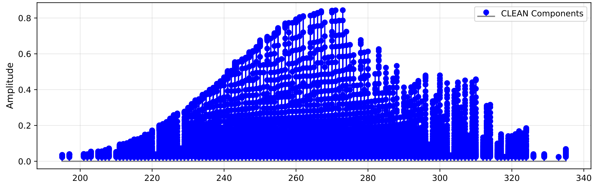
Summed CLEAN Components Profile
