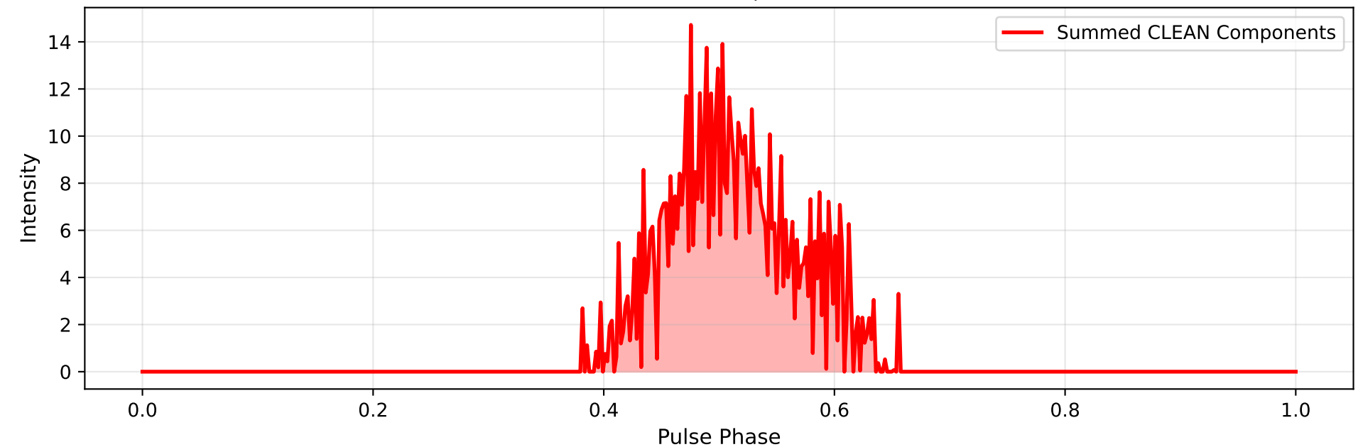
Summed CLEAN Components Profile
