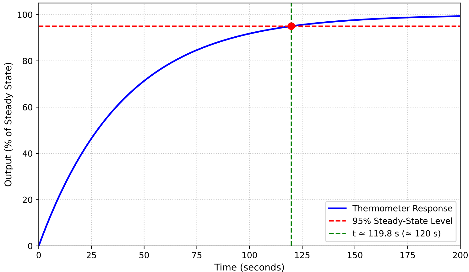
First-Order System Step Response
