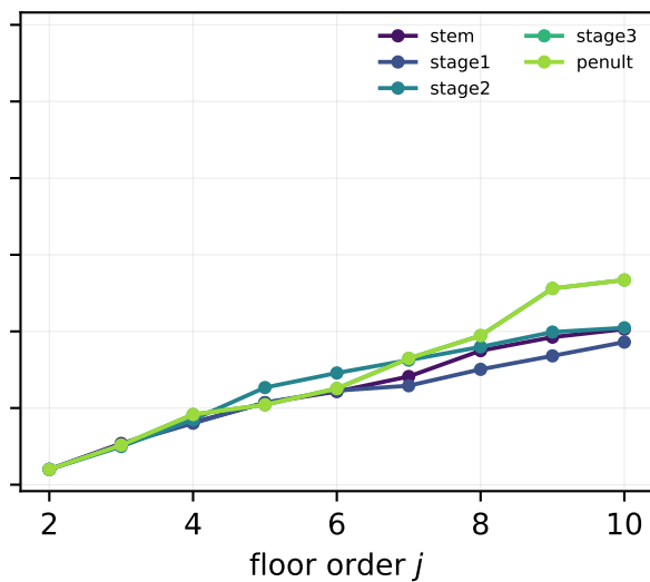
ResNet-20 / C10
