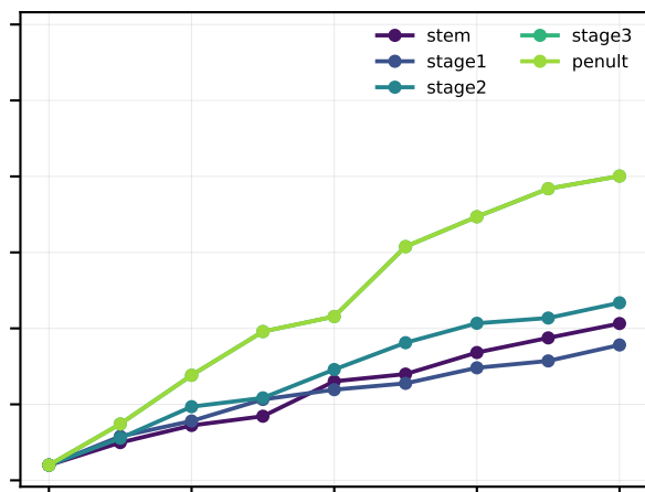
ResNet-56 / C10
