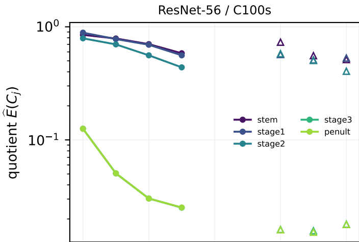
E7: the interaction spectrum decays geometrically in j , fastest in deep layers
