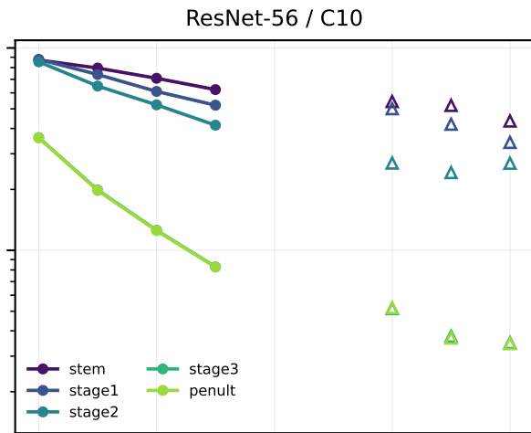
E7: the interaction spectrum decays geometrically in j , fastest in deep layers
