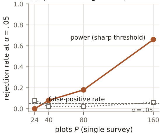
(a) power is bought with plots ...
