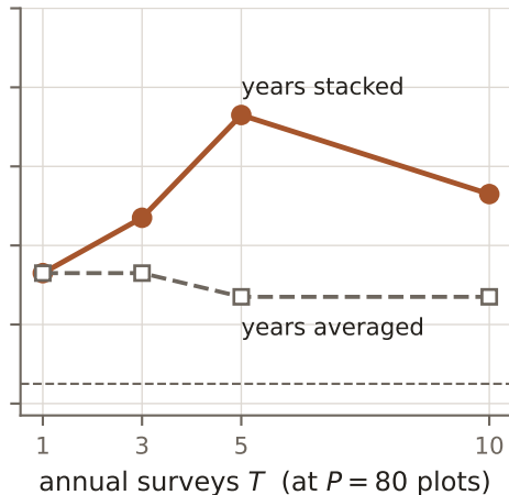
(b) ... or with repeat surveys, used correctly
