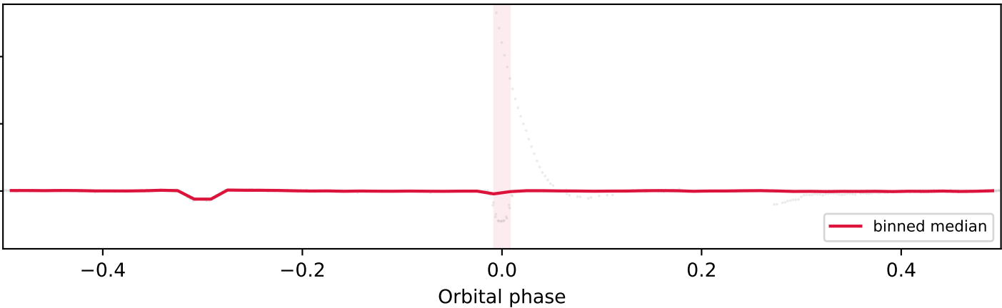
Phase-folded light curve (shaded = BLS eclipse window)
