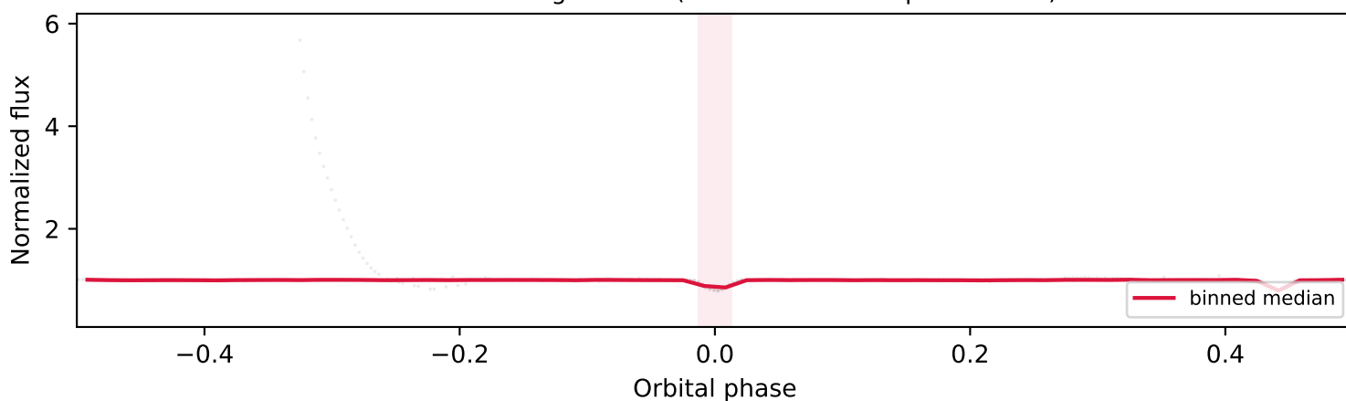
Phase-folded light curve (shaded = BLS eclipse window)
