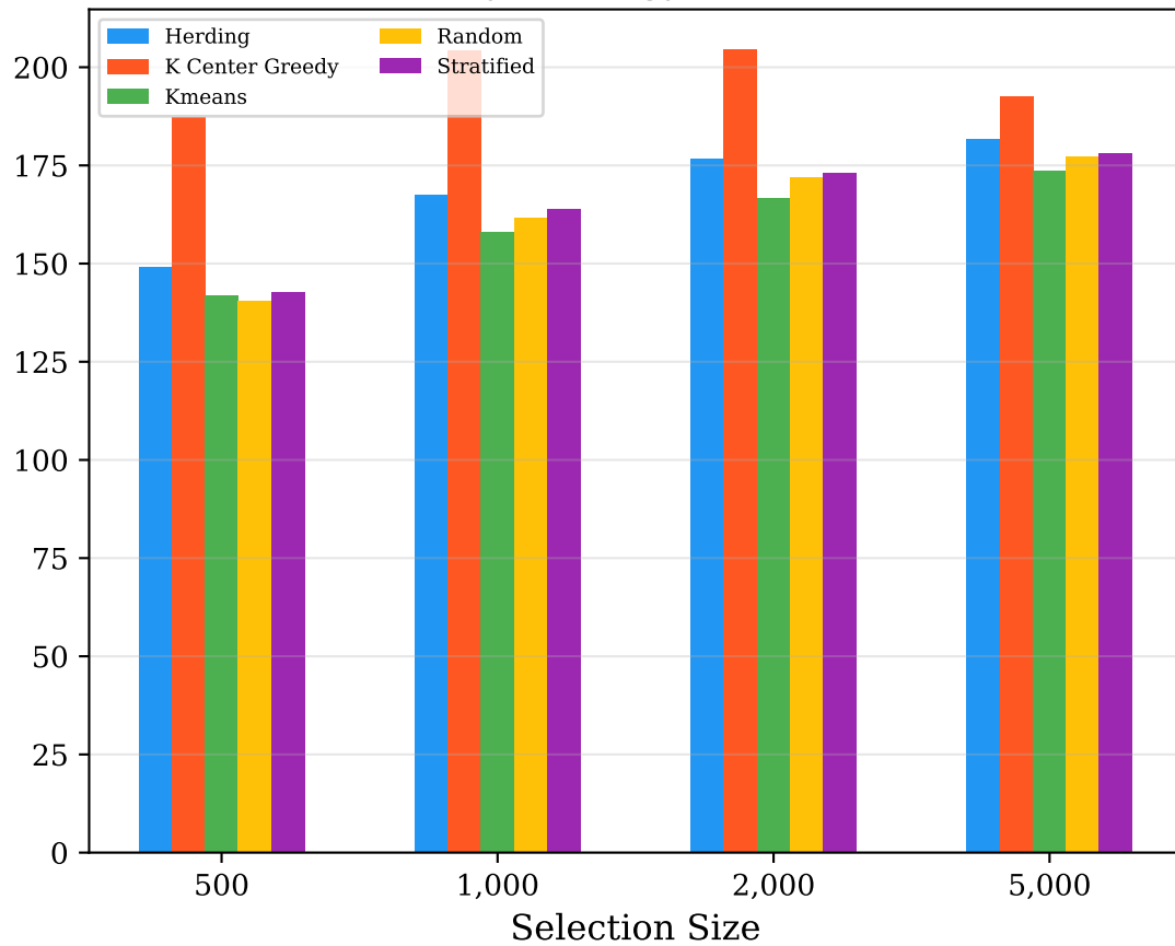
Vendi Score by Strategy and Selection Size
