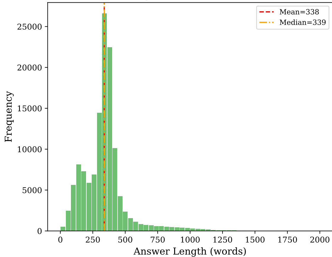
Answer Length Distribution (N=126,638)
