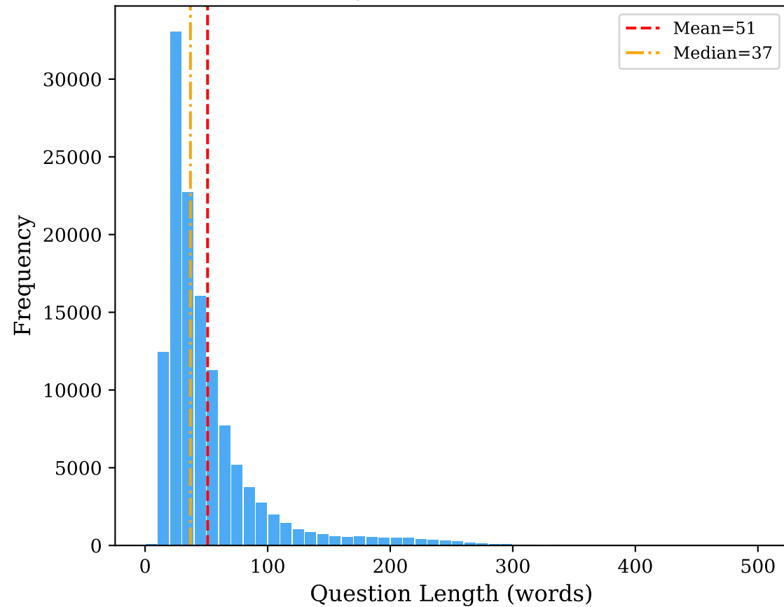
Question Length Distribution (N=126,638)
