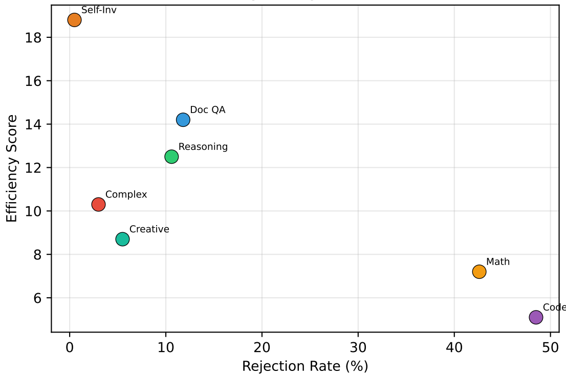
(h) Efficiency vs Rejection ( r=-0.776 )
