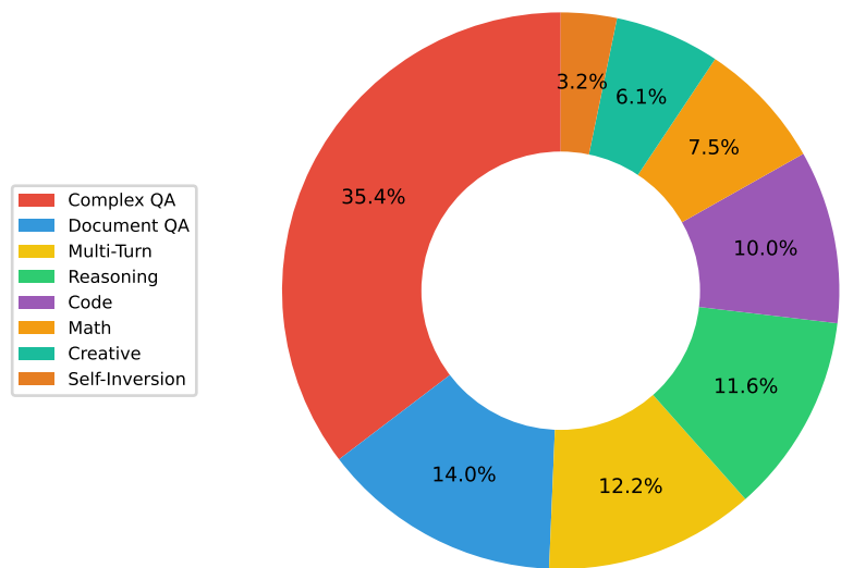
(a) 153,351 Cleaned Samples
