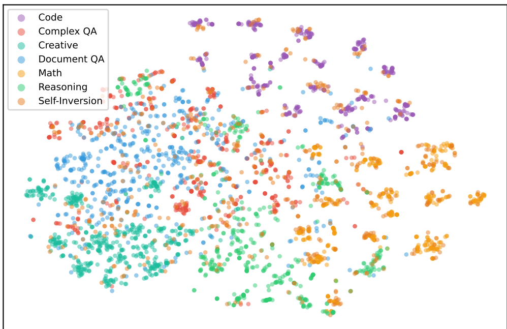
(b) Semantic Space (t-SNE)
