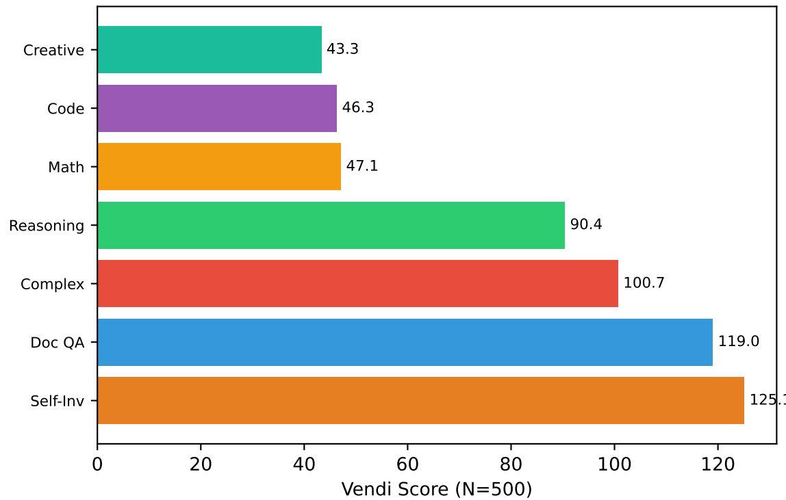
(c) Per-Pipeline Diversity
