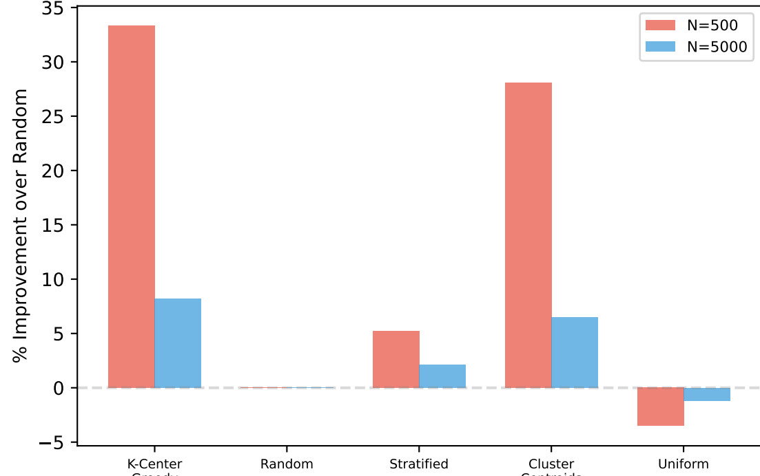
(f) Selection Strategy Impact
