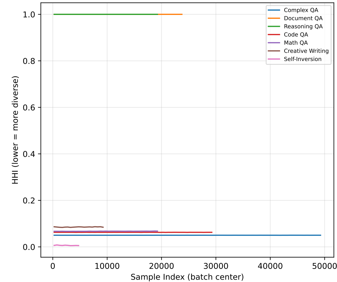
(e) Domain Concentration (HHI) per Batch
