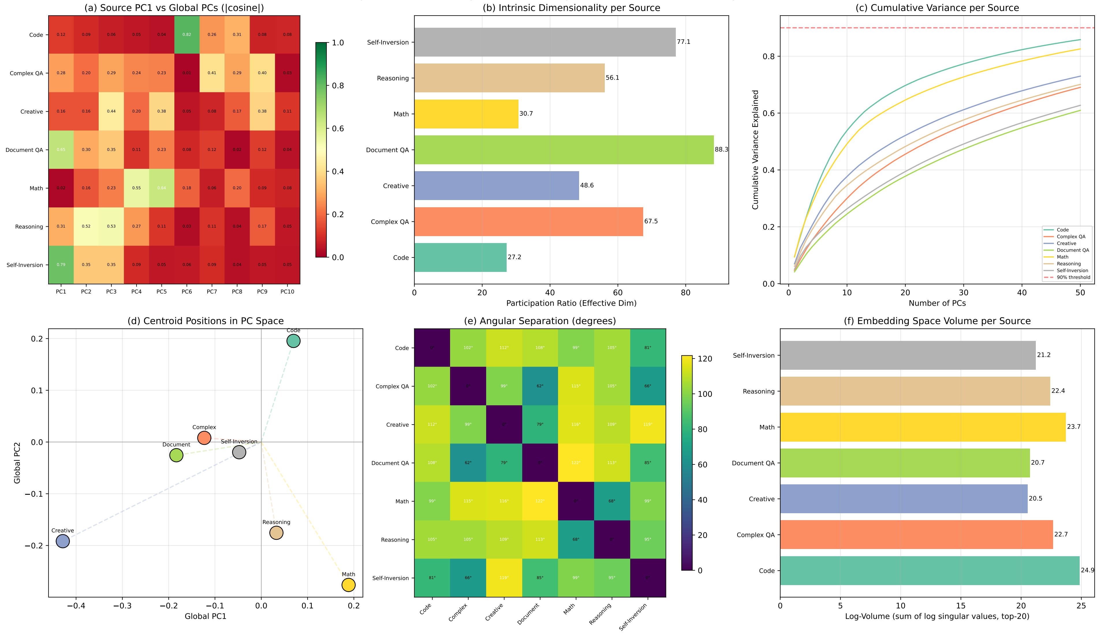
Fig 118: Embedding Subspace Alignment & Geometric Analysis
