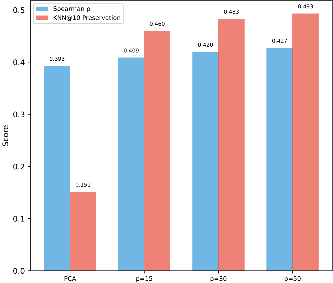
(e) Reduction Quality Comparison
