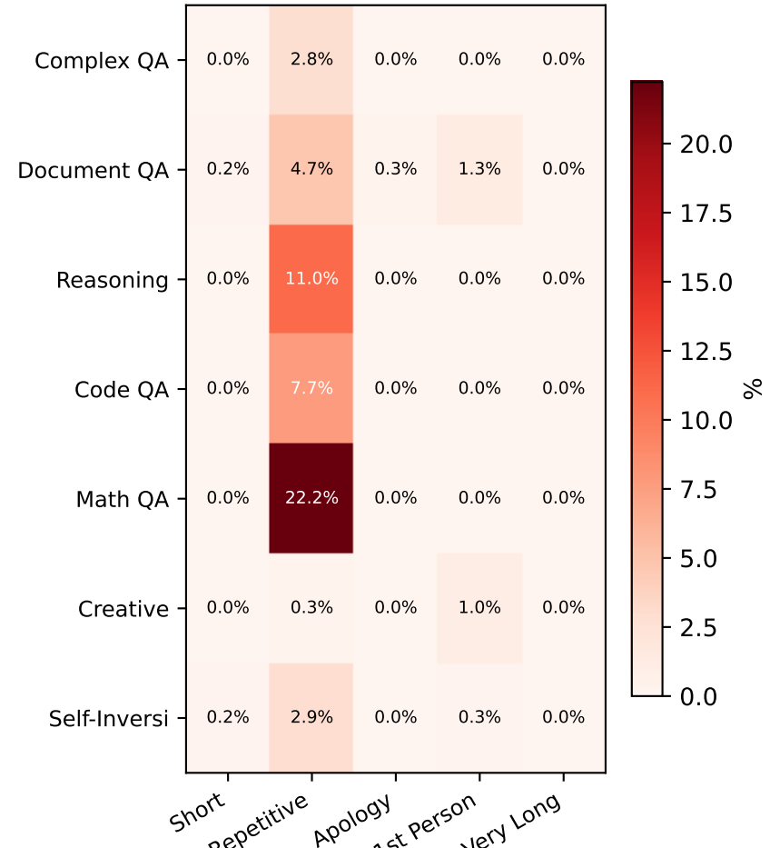
(f) Issue Heatmap
