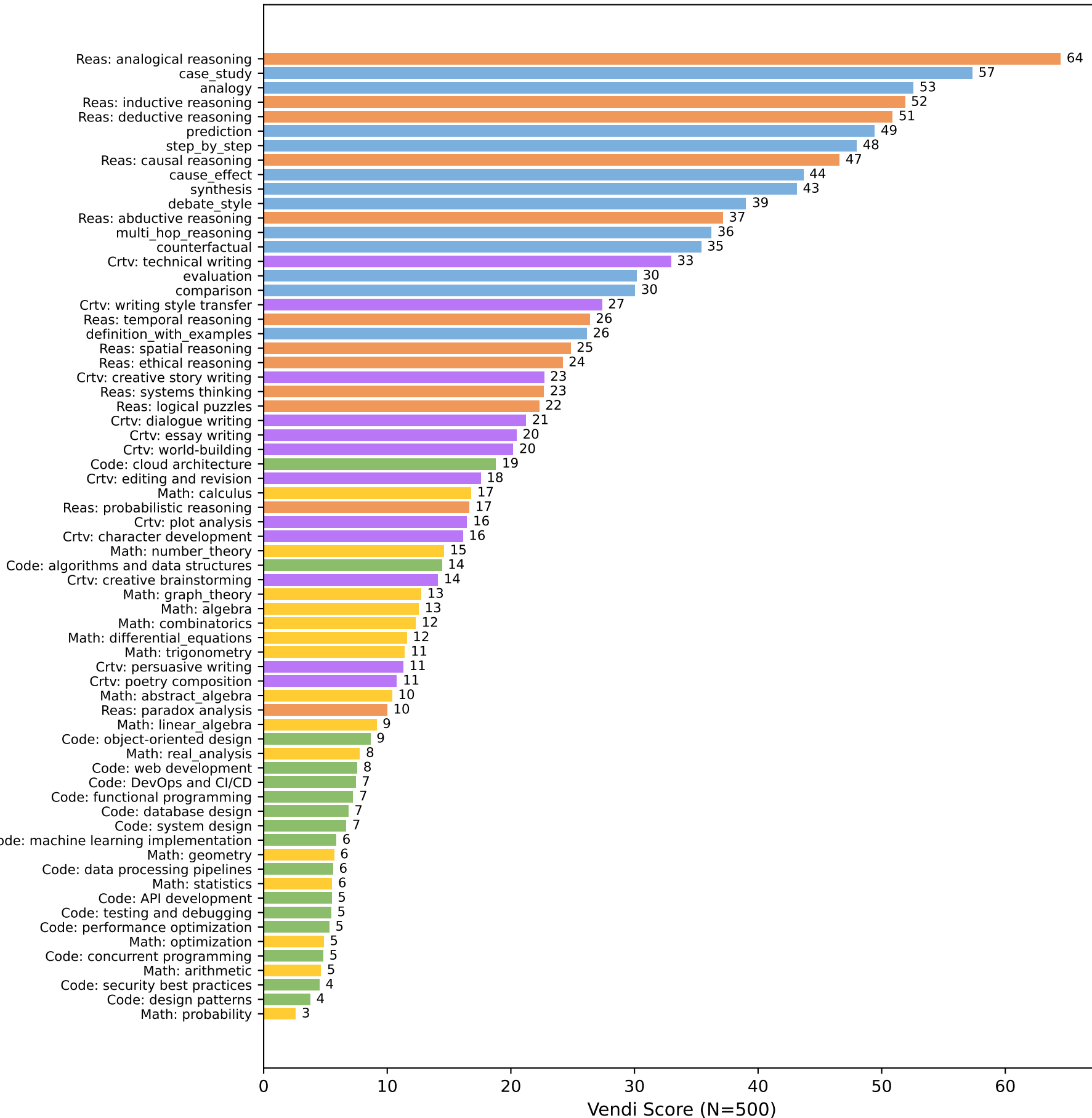
Vendi Score per Question Type
