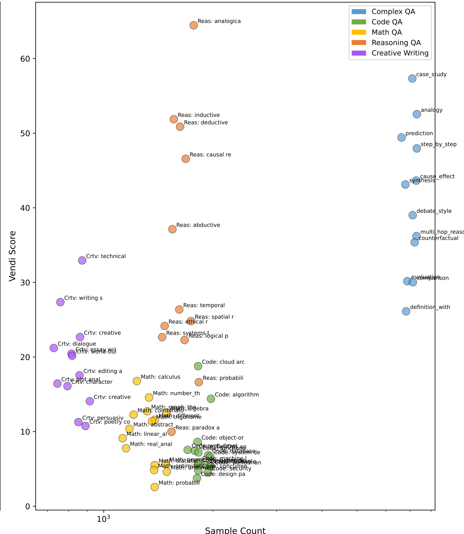
Diversity vs Volume per Type
