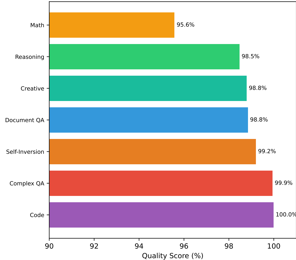
(a) Overall Quality Score
