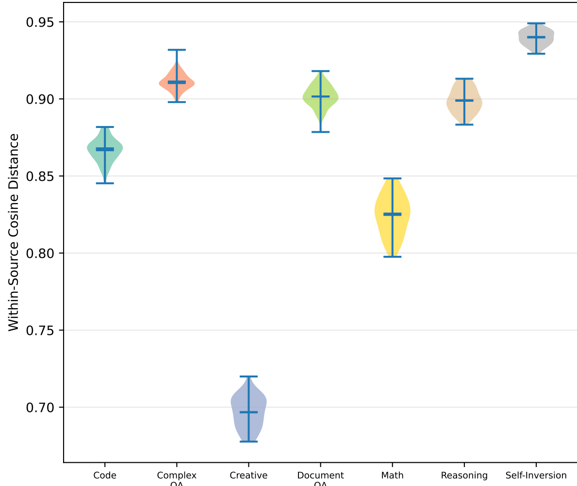
(a) Within-Source Diversity Bootstrap
