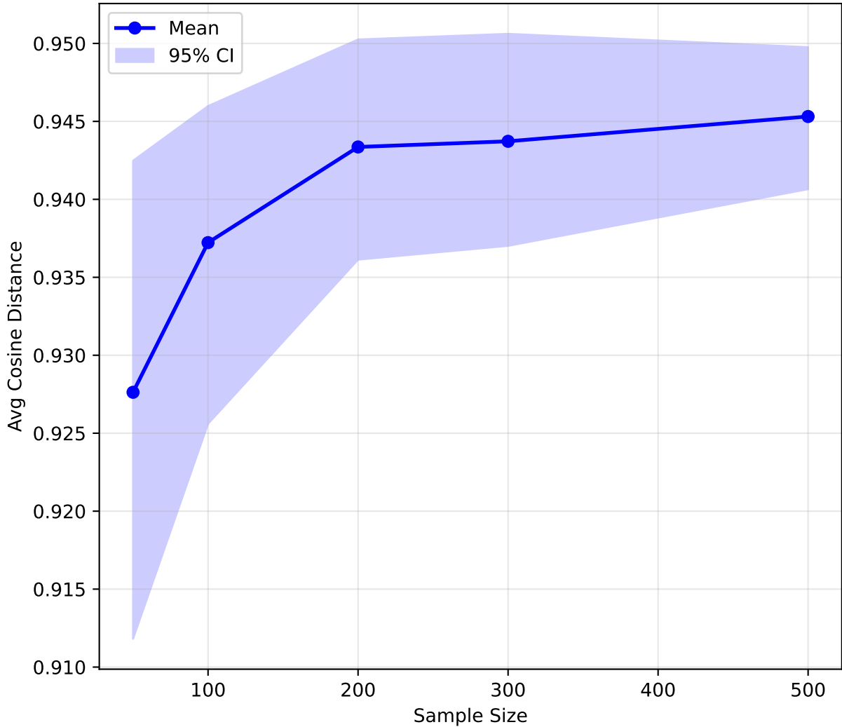
(f) Bootstrap Summary
