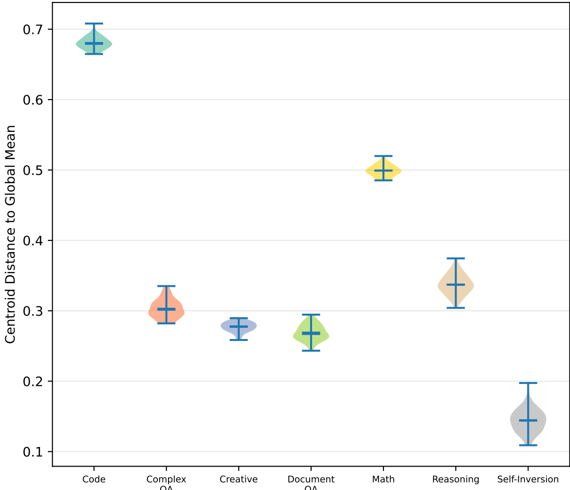
(b) Centroid Position Stability
