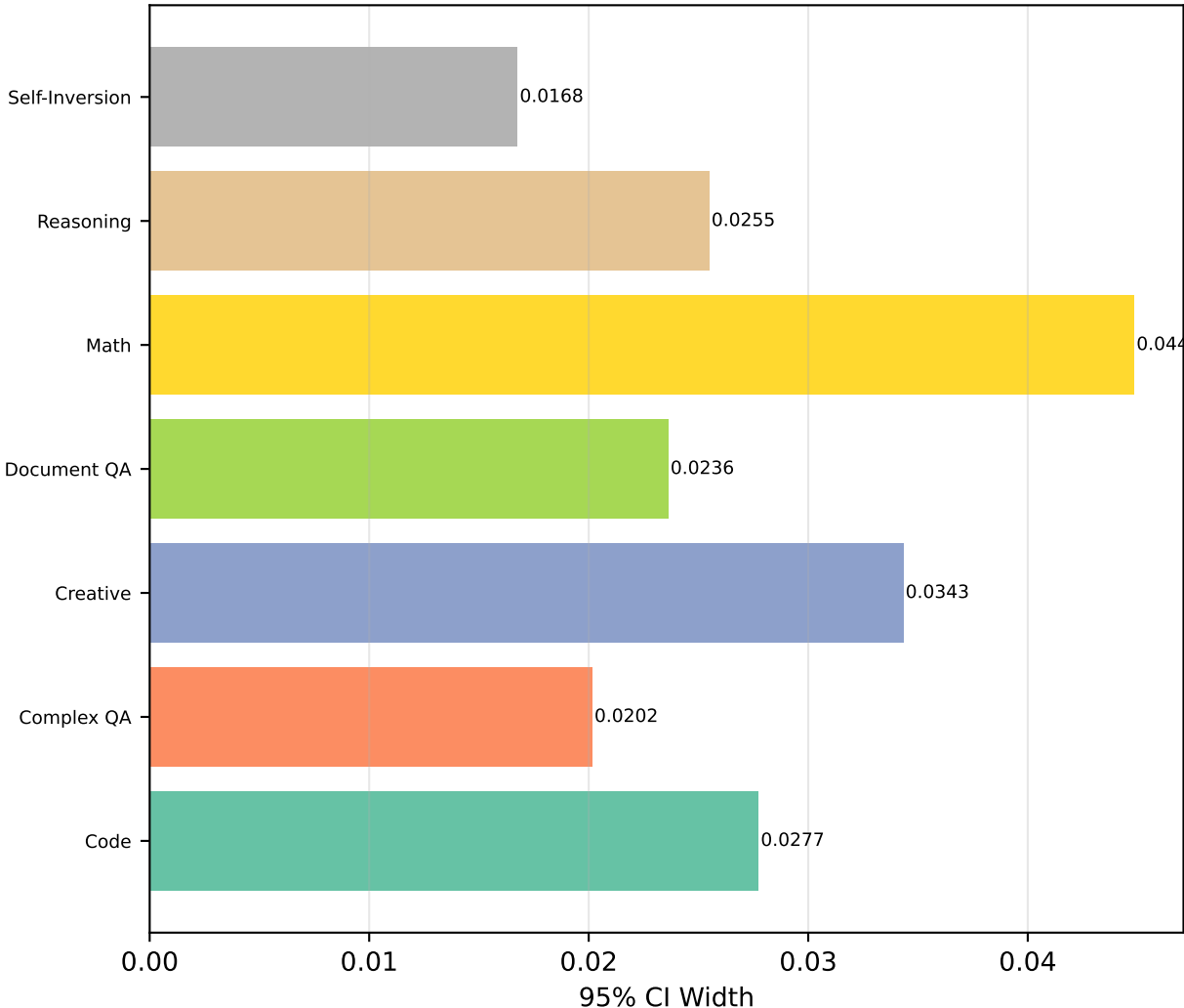
(e) Confidence Interval Width
