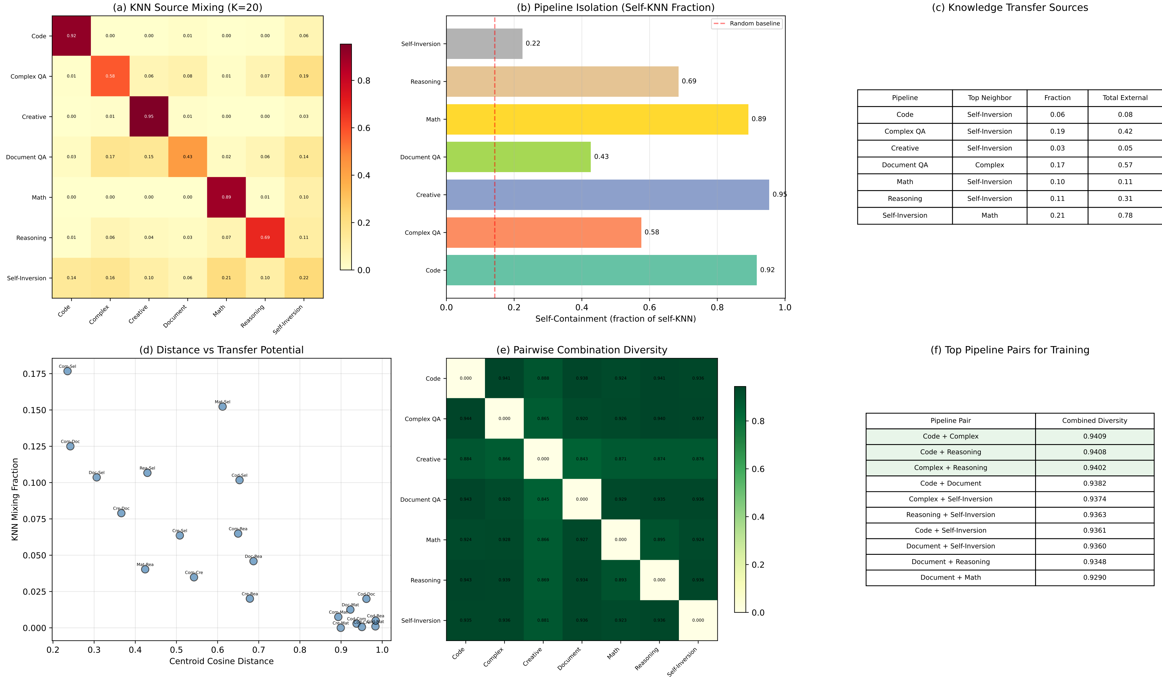
Fig 128: Cross-Pipeline Knowledge Transfer & Synergy Potential
