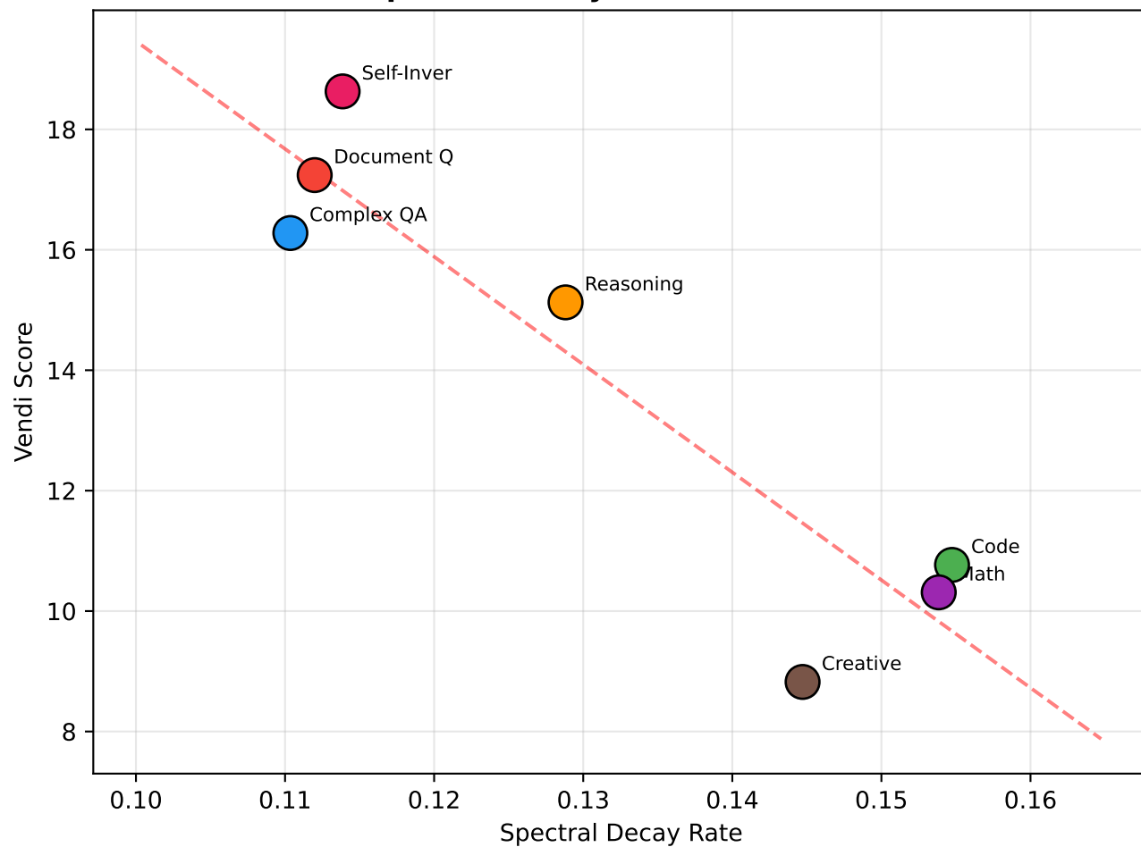
(c) Spectral Decay vs Vendi ( r=-0.921 )
