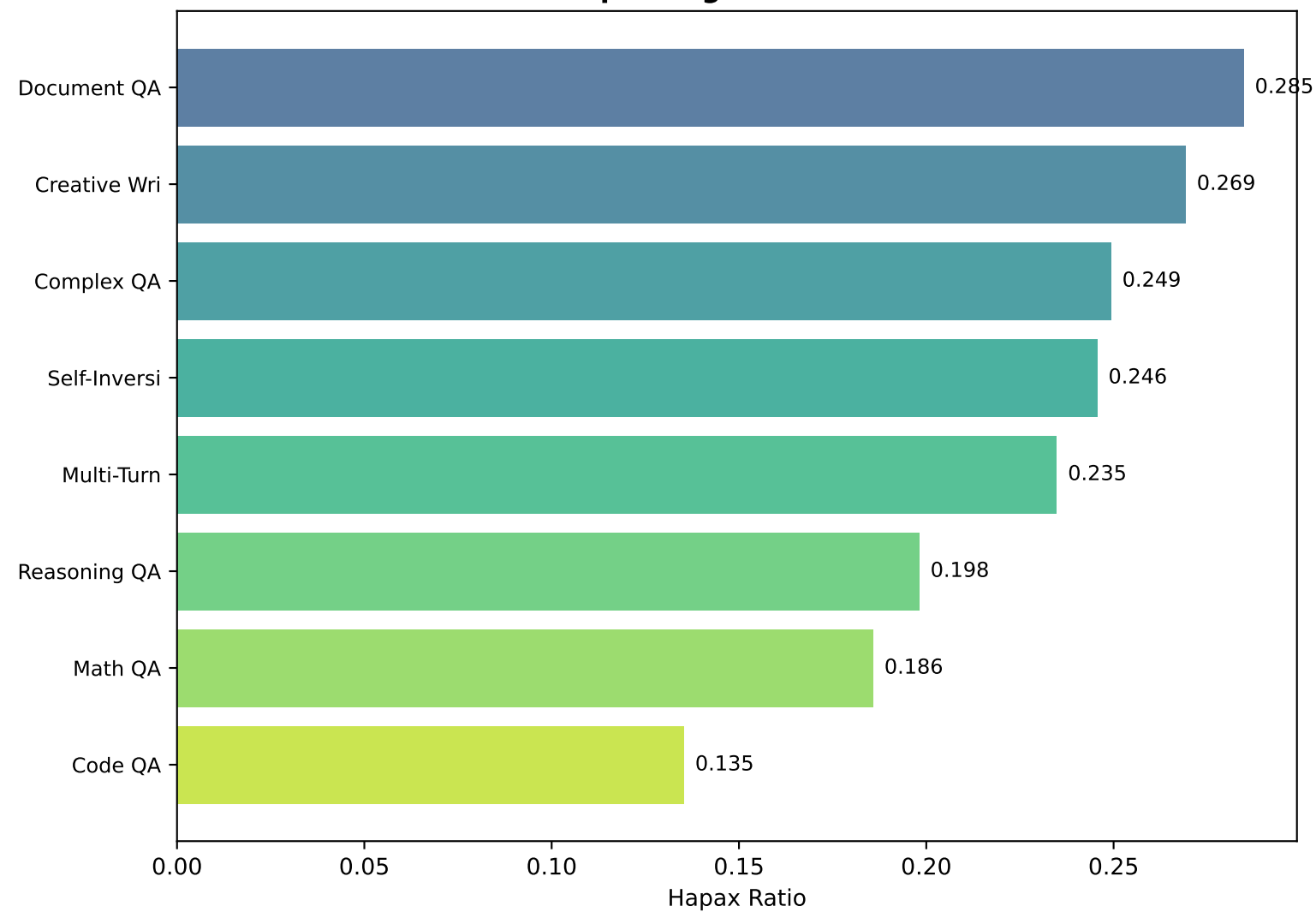
Hapax Legomena Ratio
