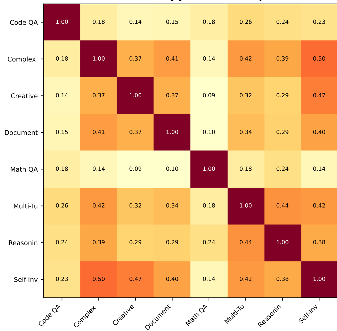
Vocabulary Jaccard Overlap
