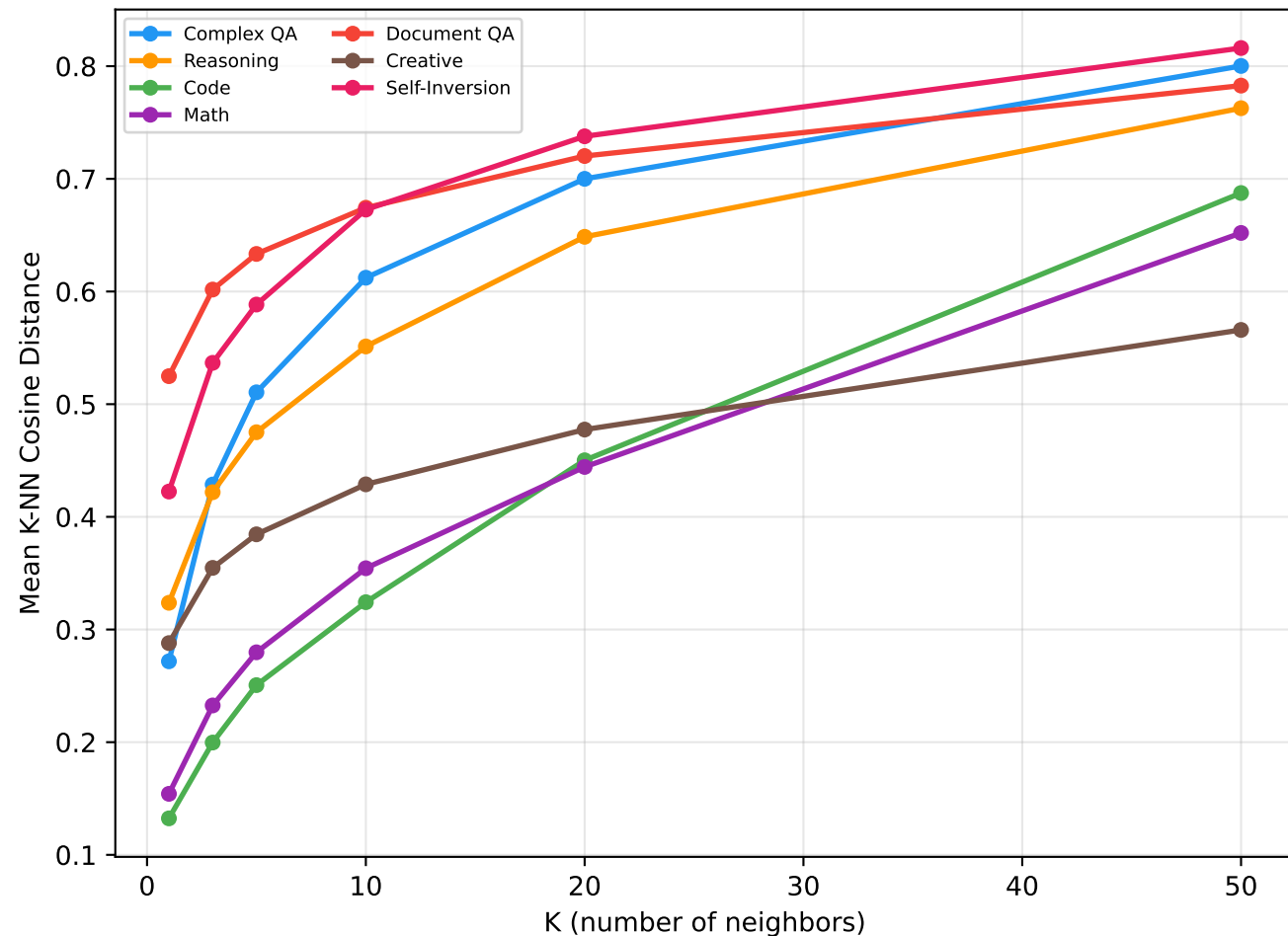
(c) K-NN Distance Growth Curve
