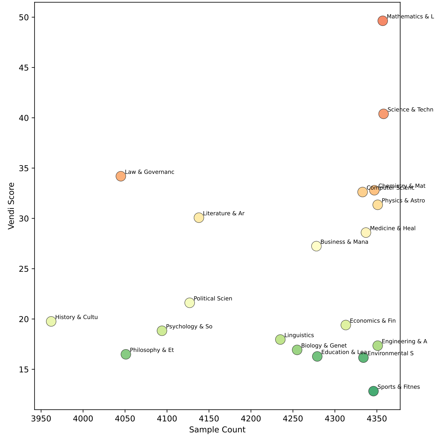
Domain Size vs Diversity
