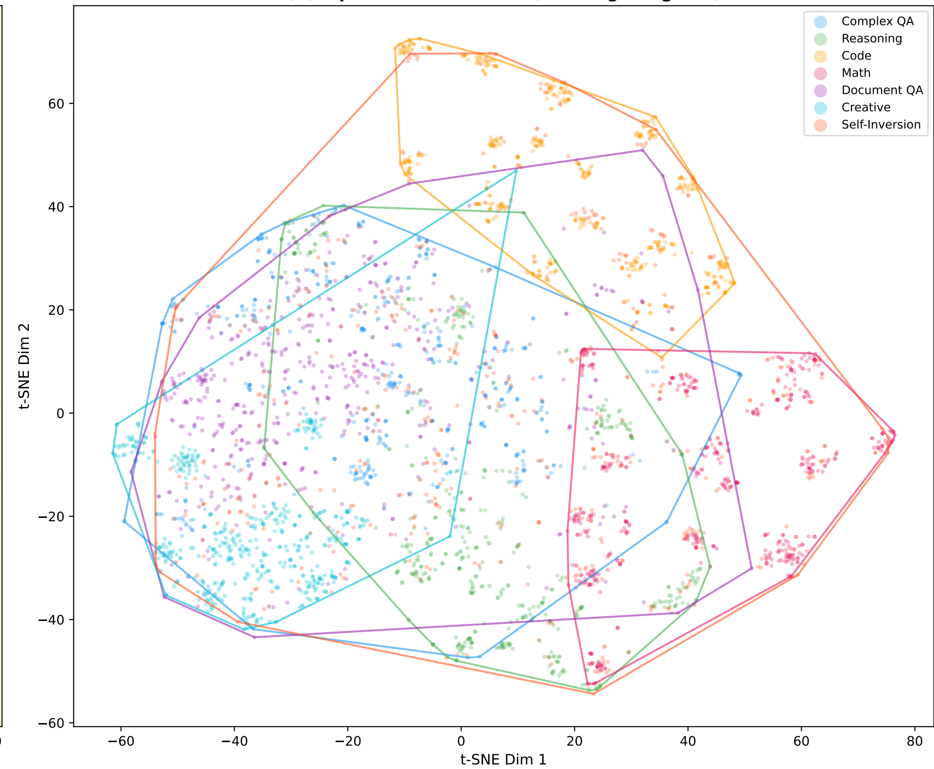
(b) Pipeline Convex Hulls (Coverage Regions)
