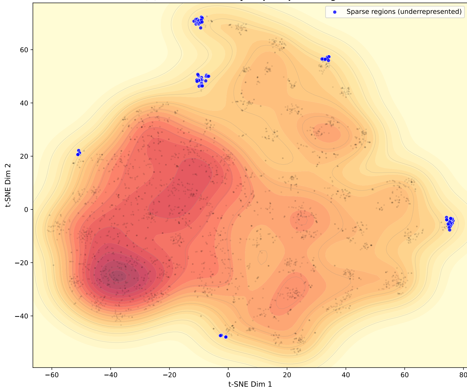
(a) Semantic Density Map + Sparse Regions
