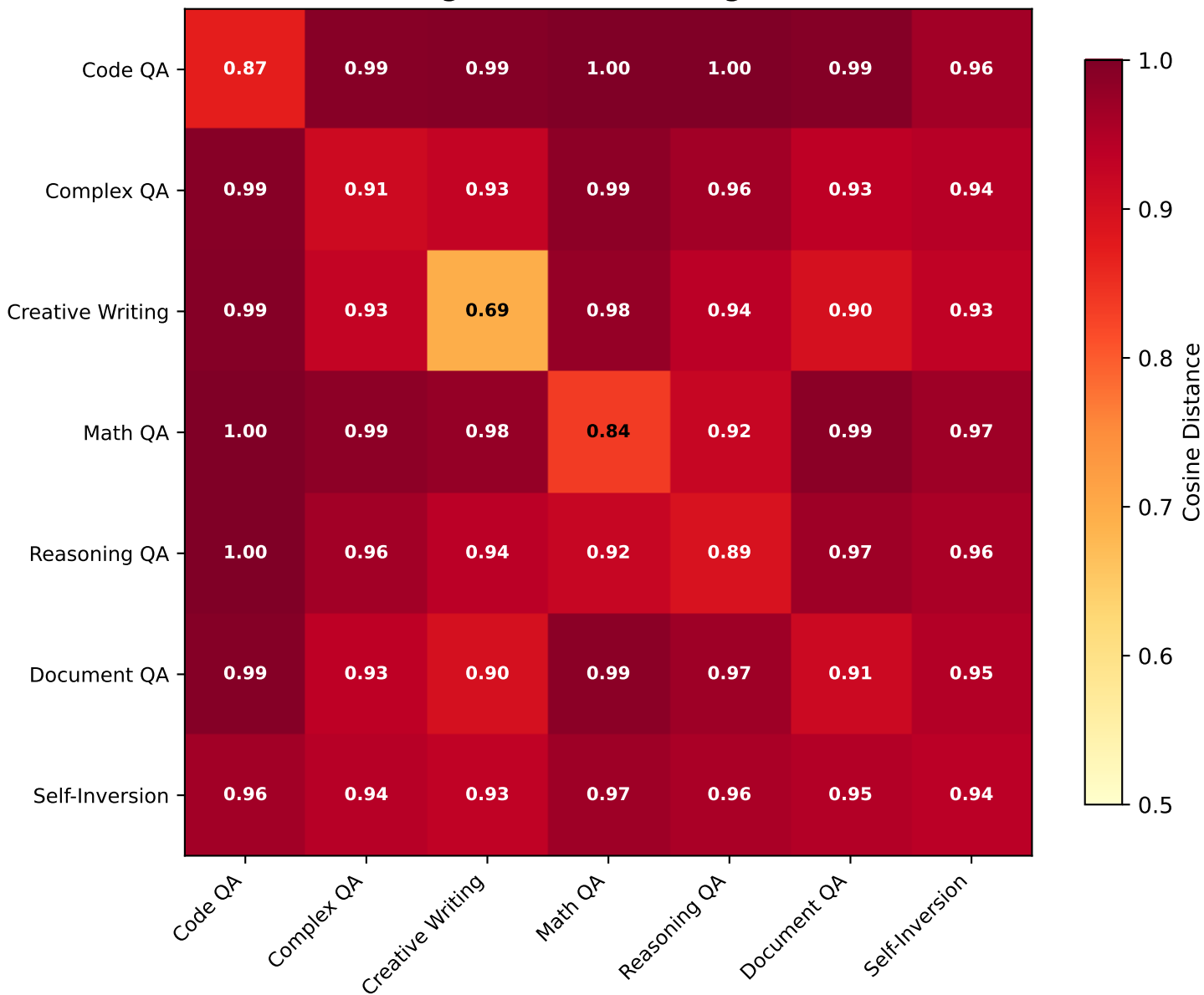
Cross-Source Embedding Distance (Higher = More Orthogonal)
