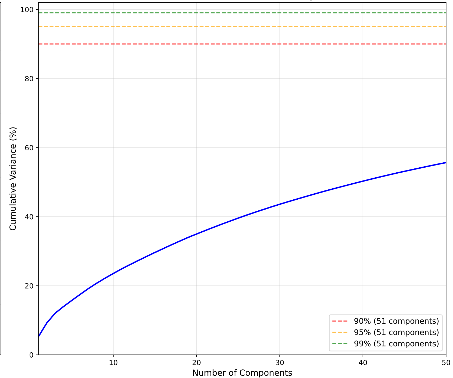
(b) PCA Cumulative Variance Explained
