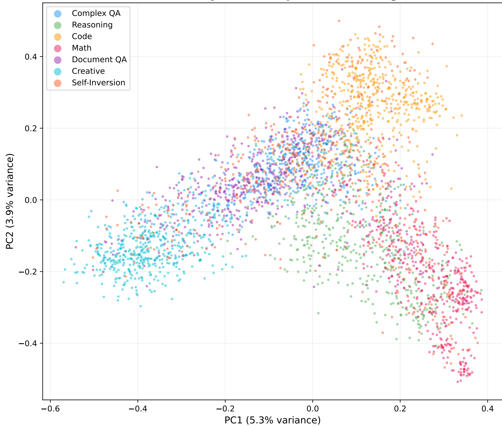
(a) PCA Projection of Pipeline Embeddings
