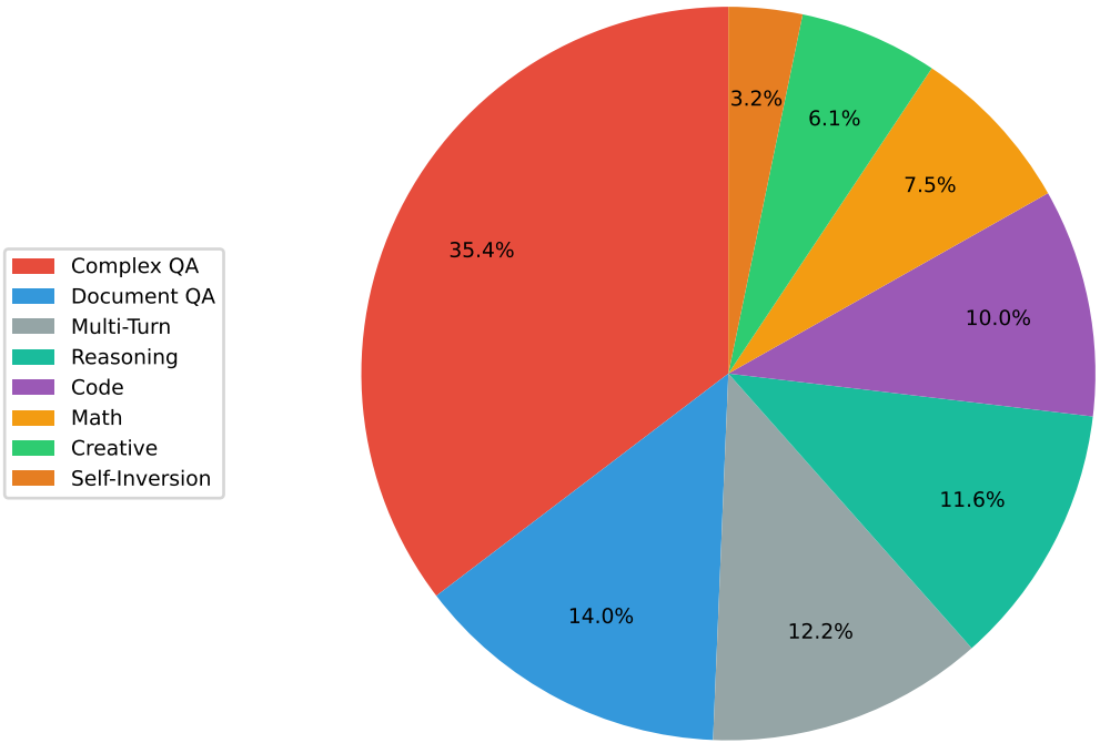
(a) Dataset Composition (153,351)
