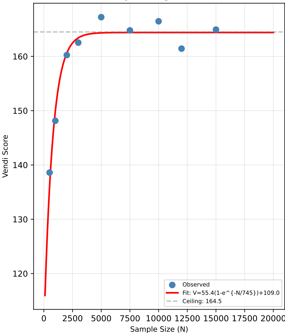
(e) Diversity Scaling Law ( R^2=0.996 )
