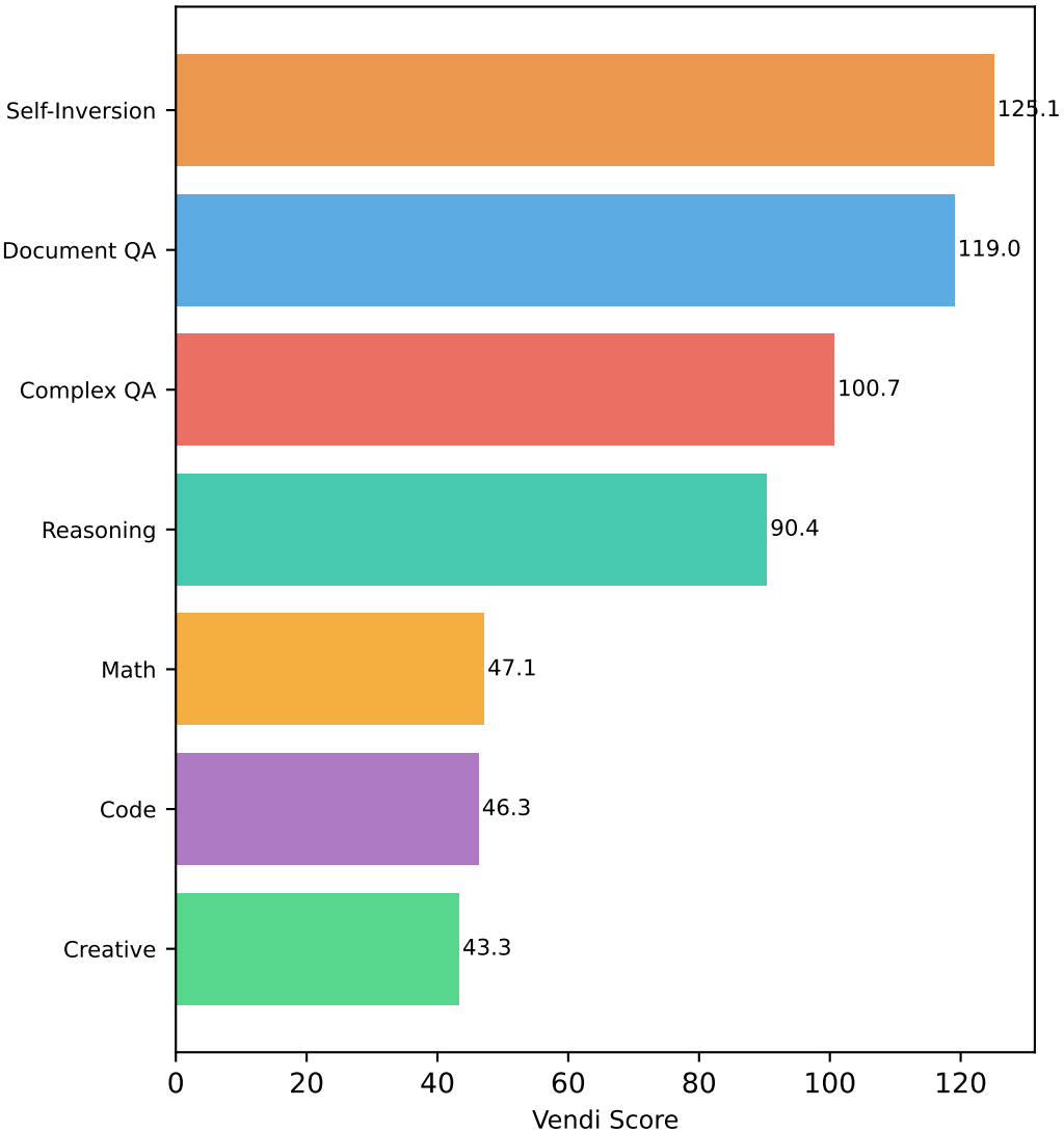
(c) Per-Pipeline Diversity
