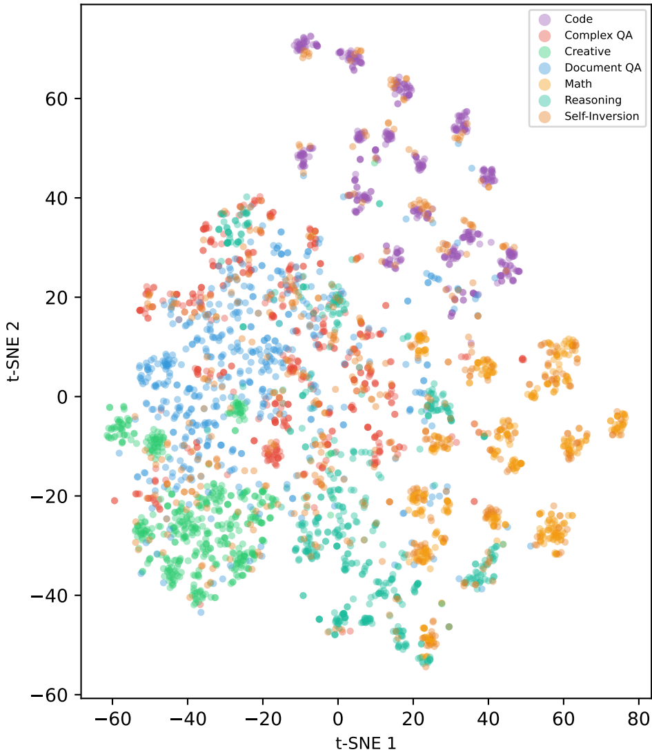
(b) Embedding Space (7 Pipelines)
