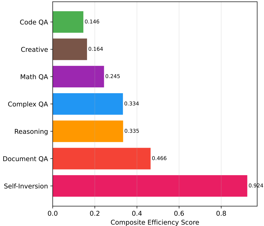
(e) Overall Efficiency Ranking
