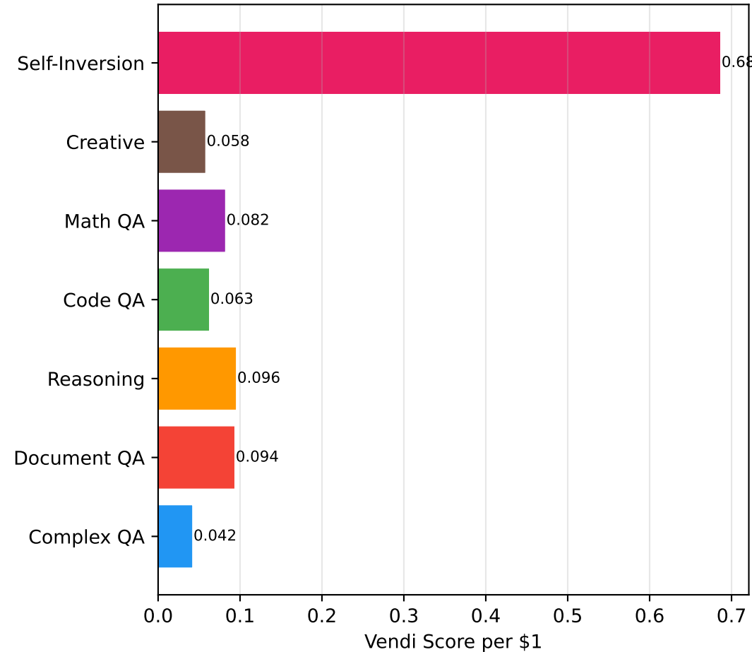
(a) Diversity per Dollar
