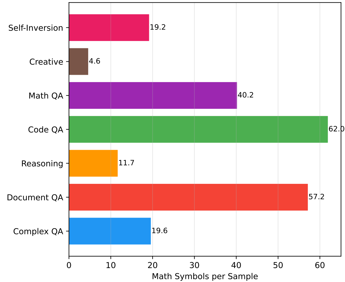
(e) Math Symbol Density
