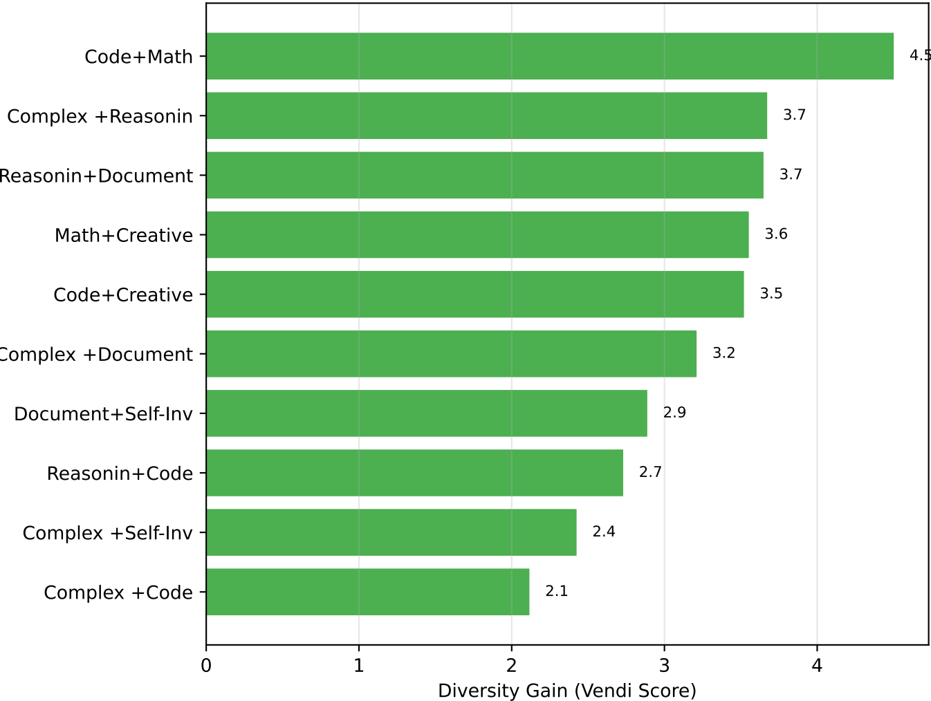
(c) Top Synergistic Pairs
