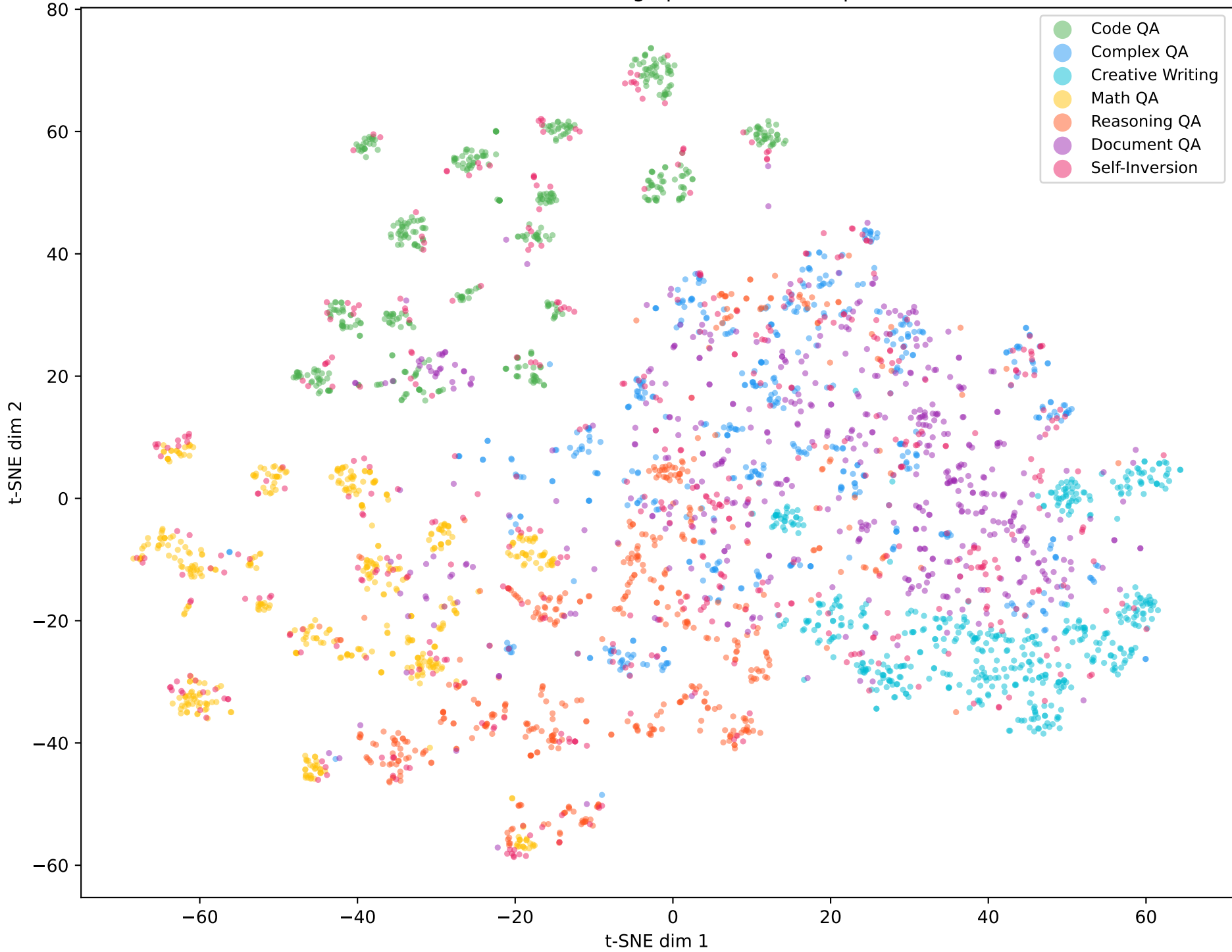
t-SNE of FANNO-Dev Embedding Space (3,500 samples, 7 sources)
