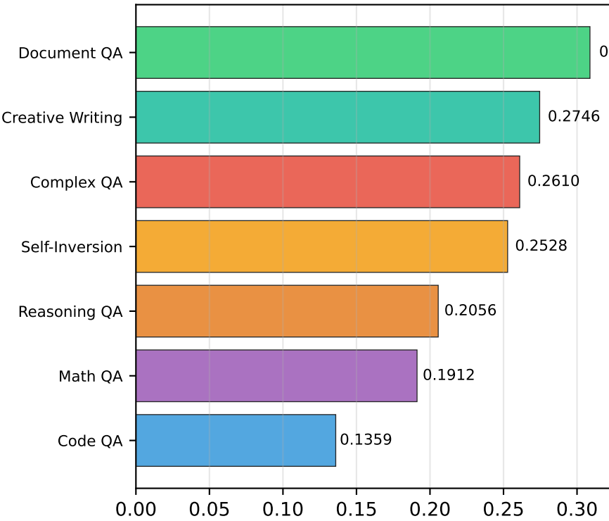
Hapax Ratio (Uniqueness)
