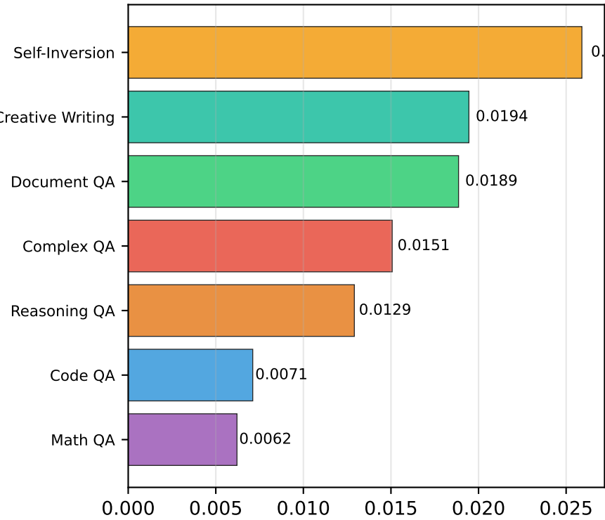
TTR (Vocab Density)
