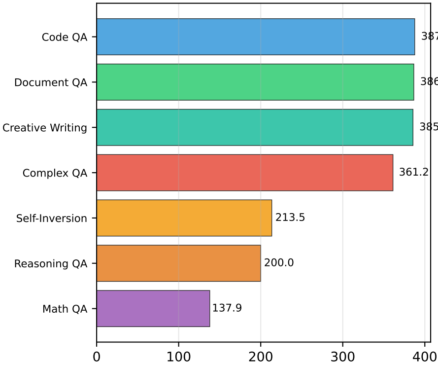
Avg Length (Words)
