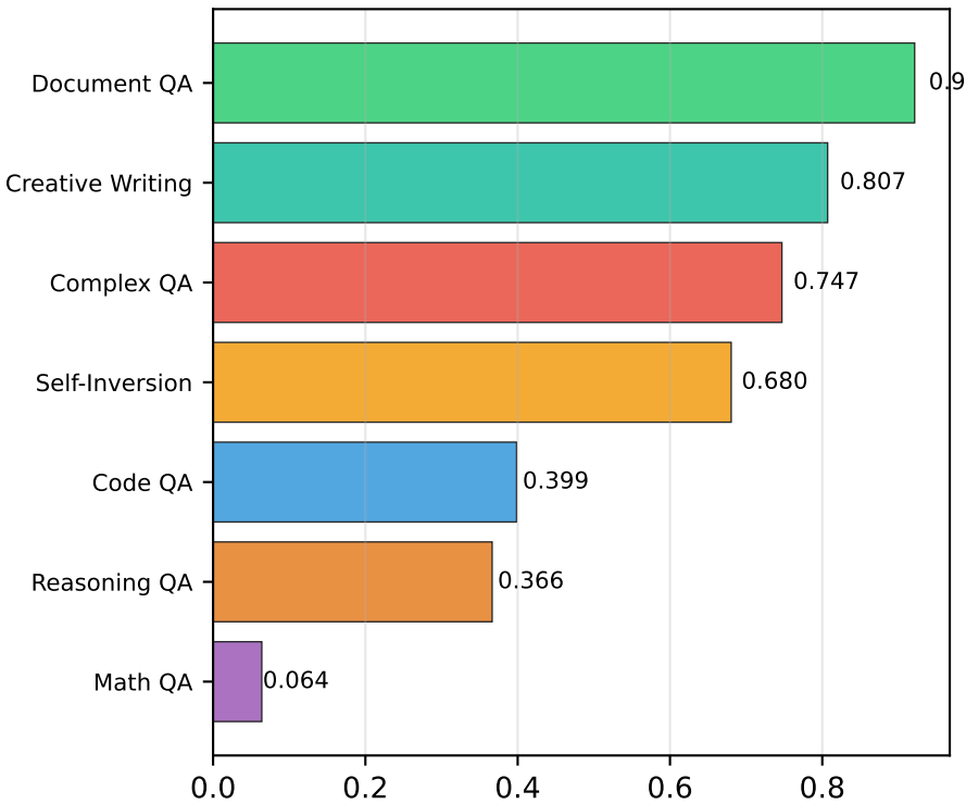
Composite Score (Normalized Average)
