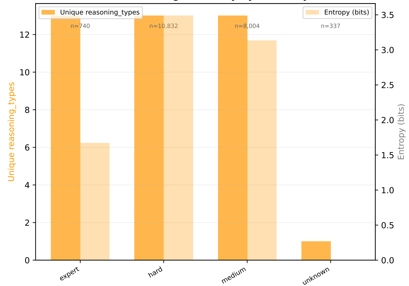
(b) Reasoning: Diversity by Difficulty
