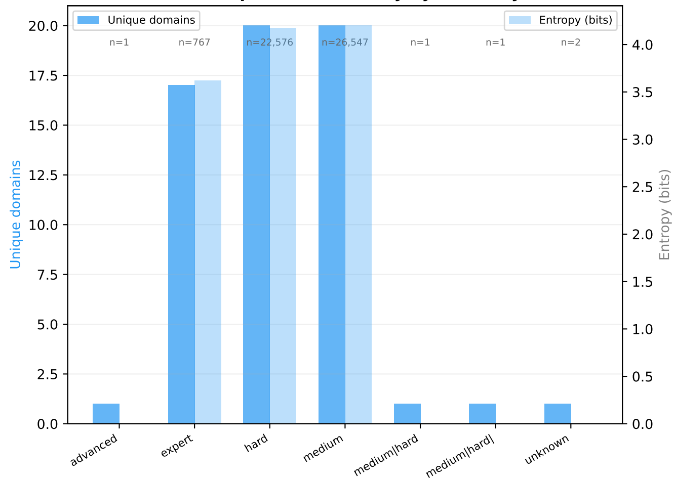
(c) Code QA: Diversity by Difficulty
