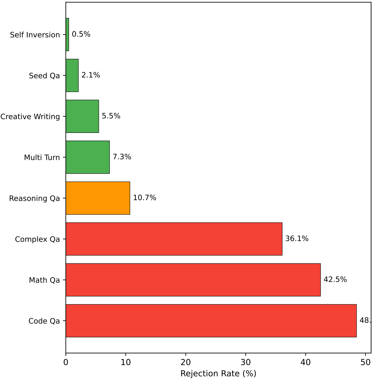
Per-Pipeline Rejection Rates
