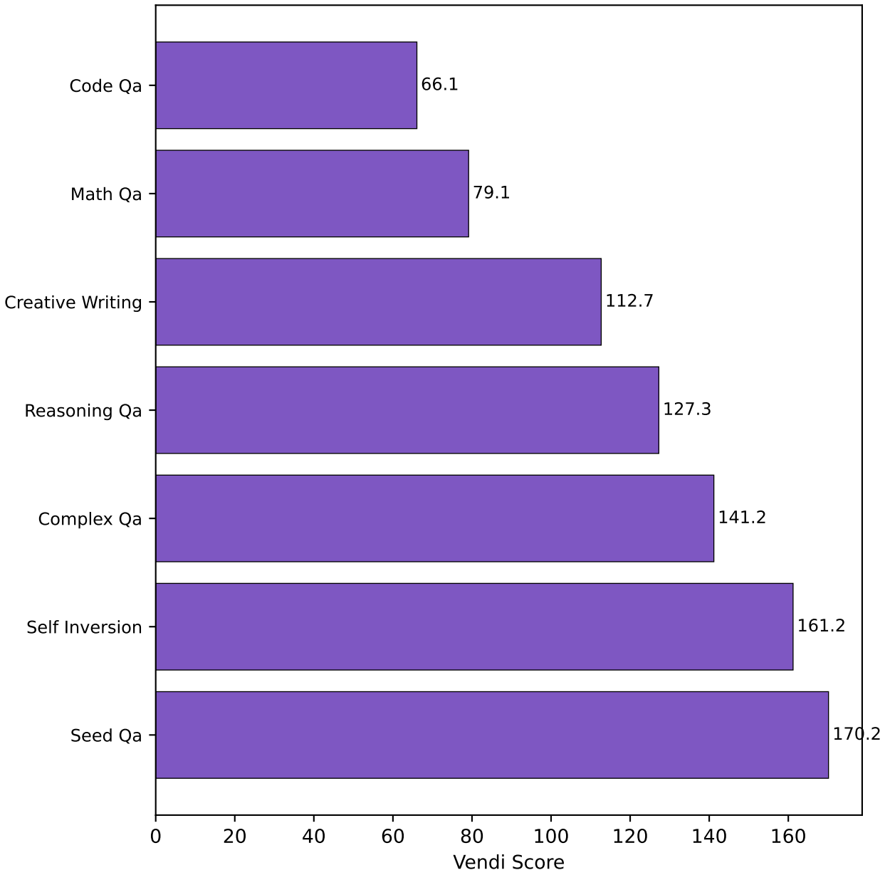
Per-Pipeline Vendi Diversity
