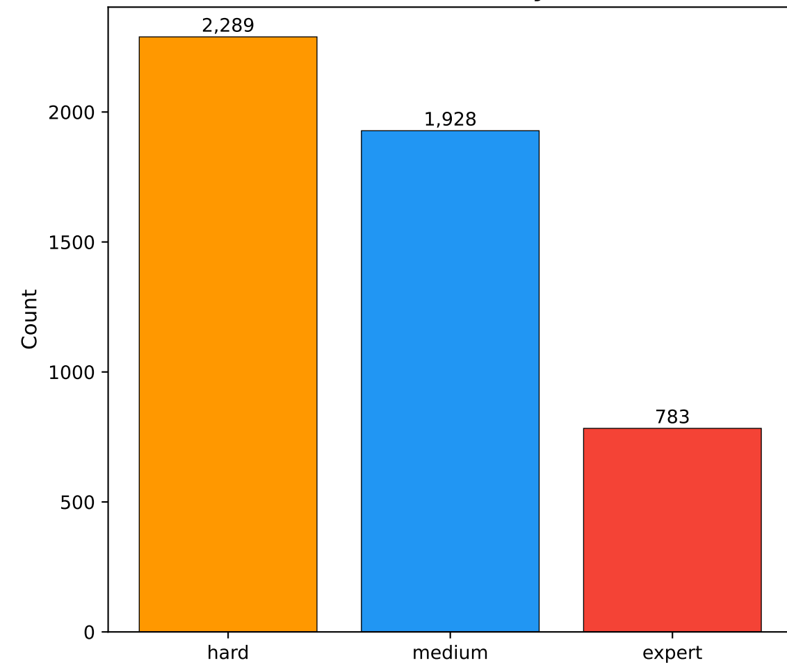
(c) Self-Inversion Difficulty Distribution
