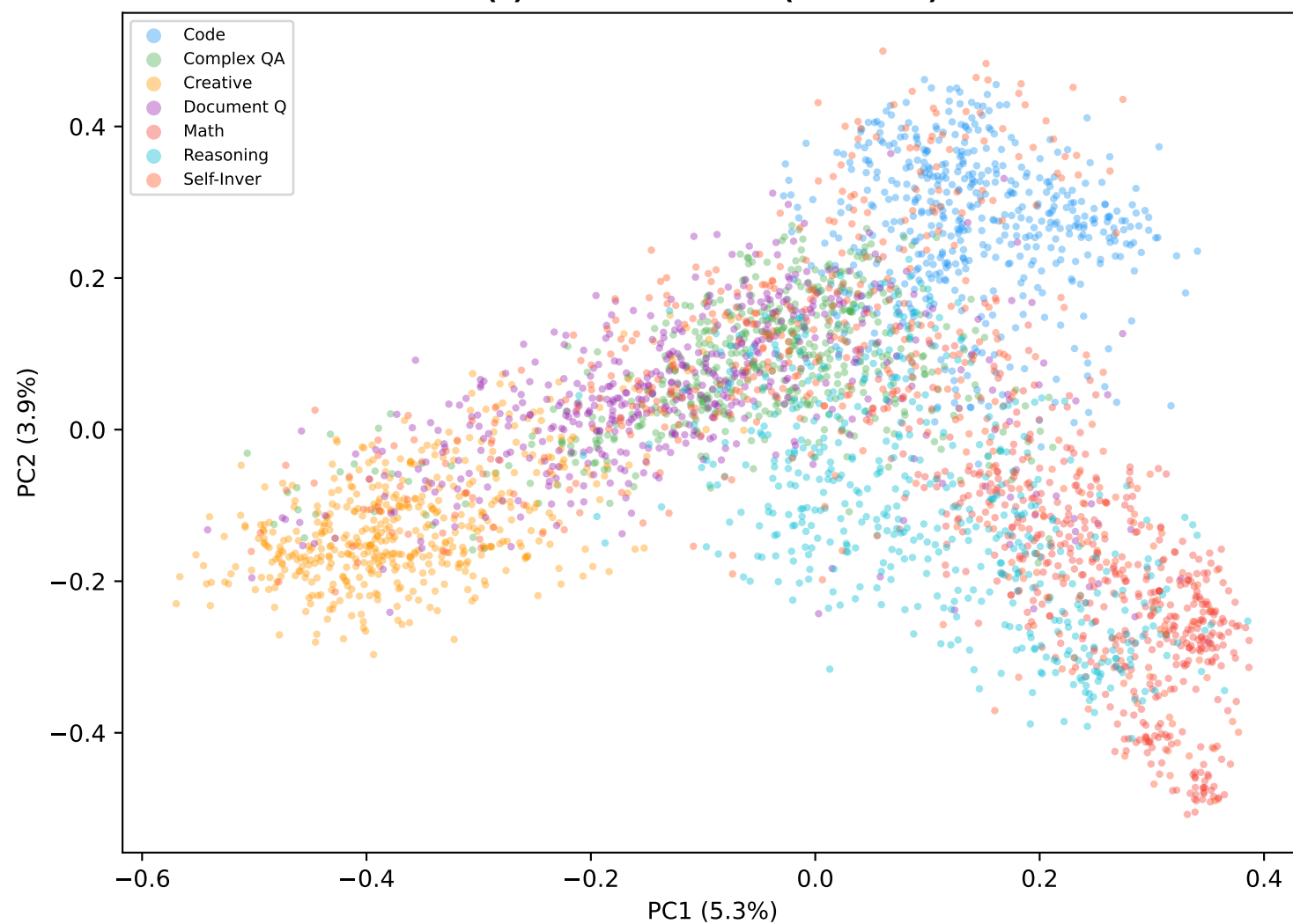
(c) PCA: PC1 vs PC2 (Centered)
