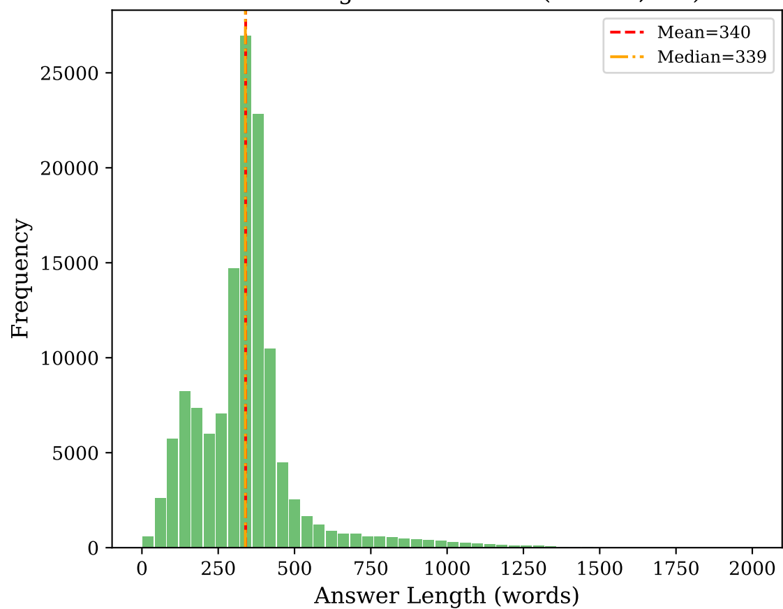
Answer Length Distribution (N=129,634)
