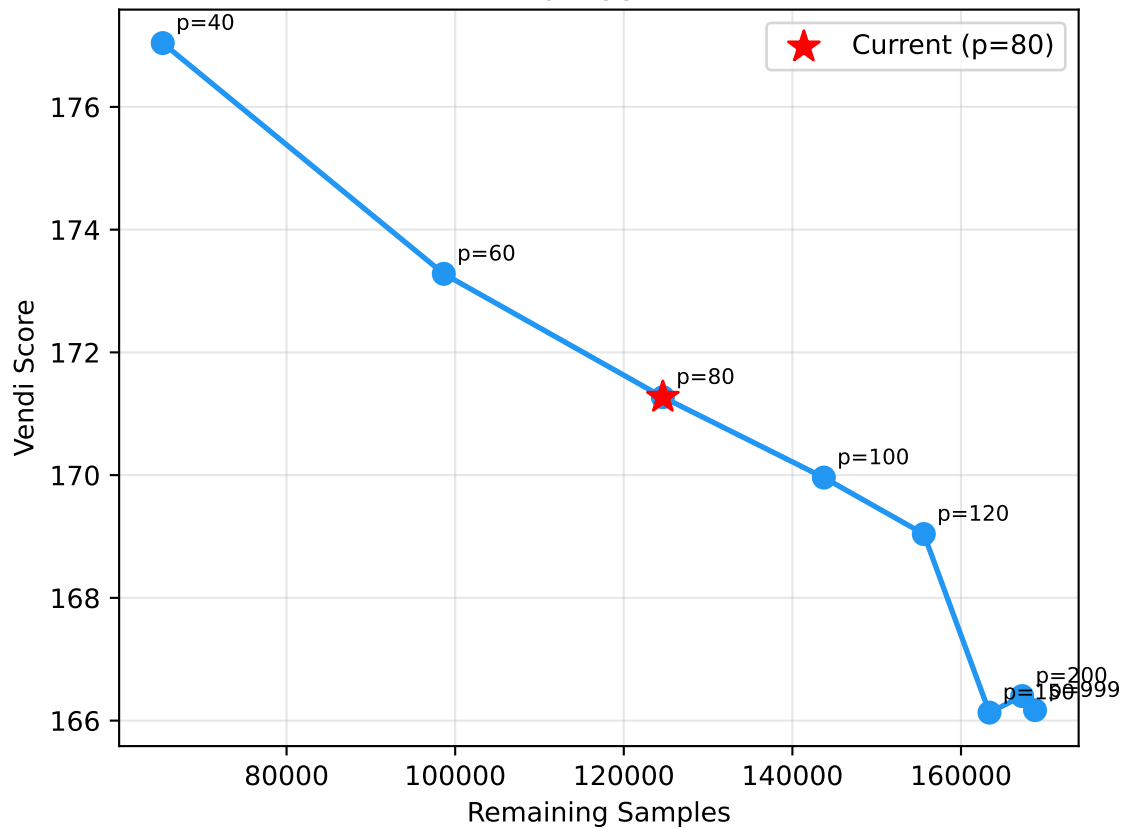
Diversity vs. Data Quantity (Near-Dedup Aggressiveness)
