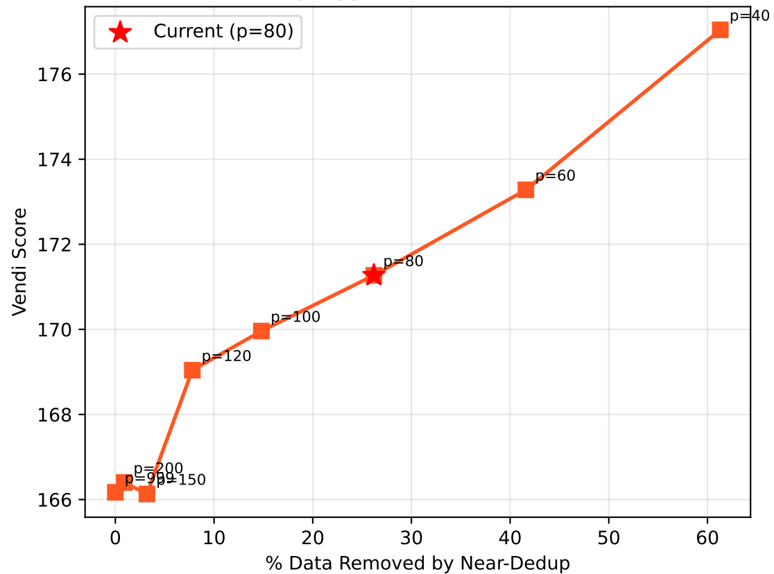
Dedup Aggressiveness Trade-off
