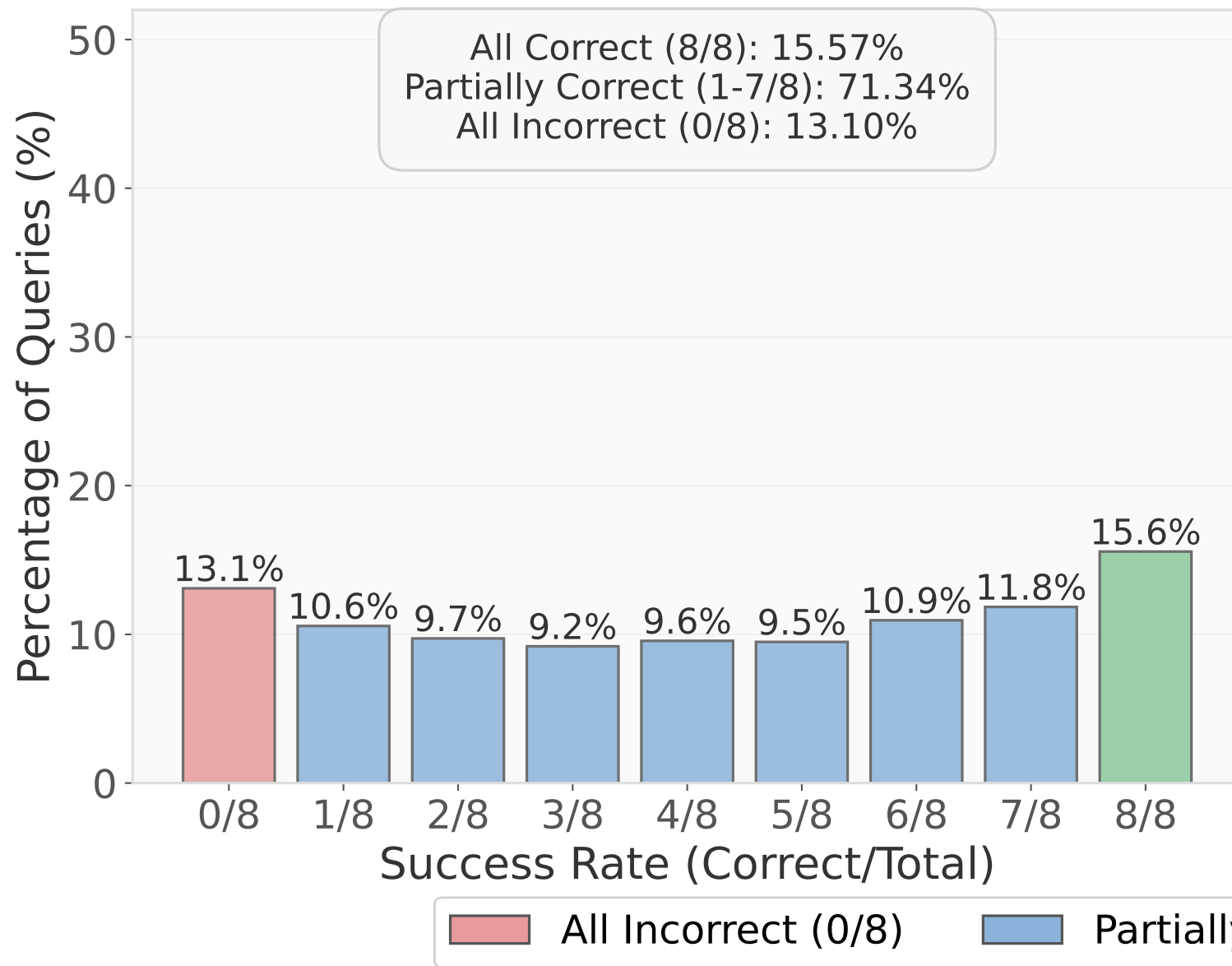
Qwen3.5-35B-A3B
