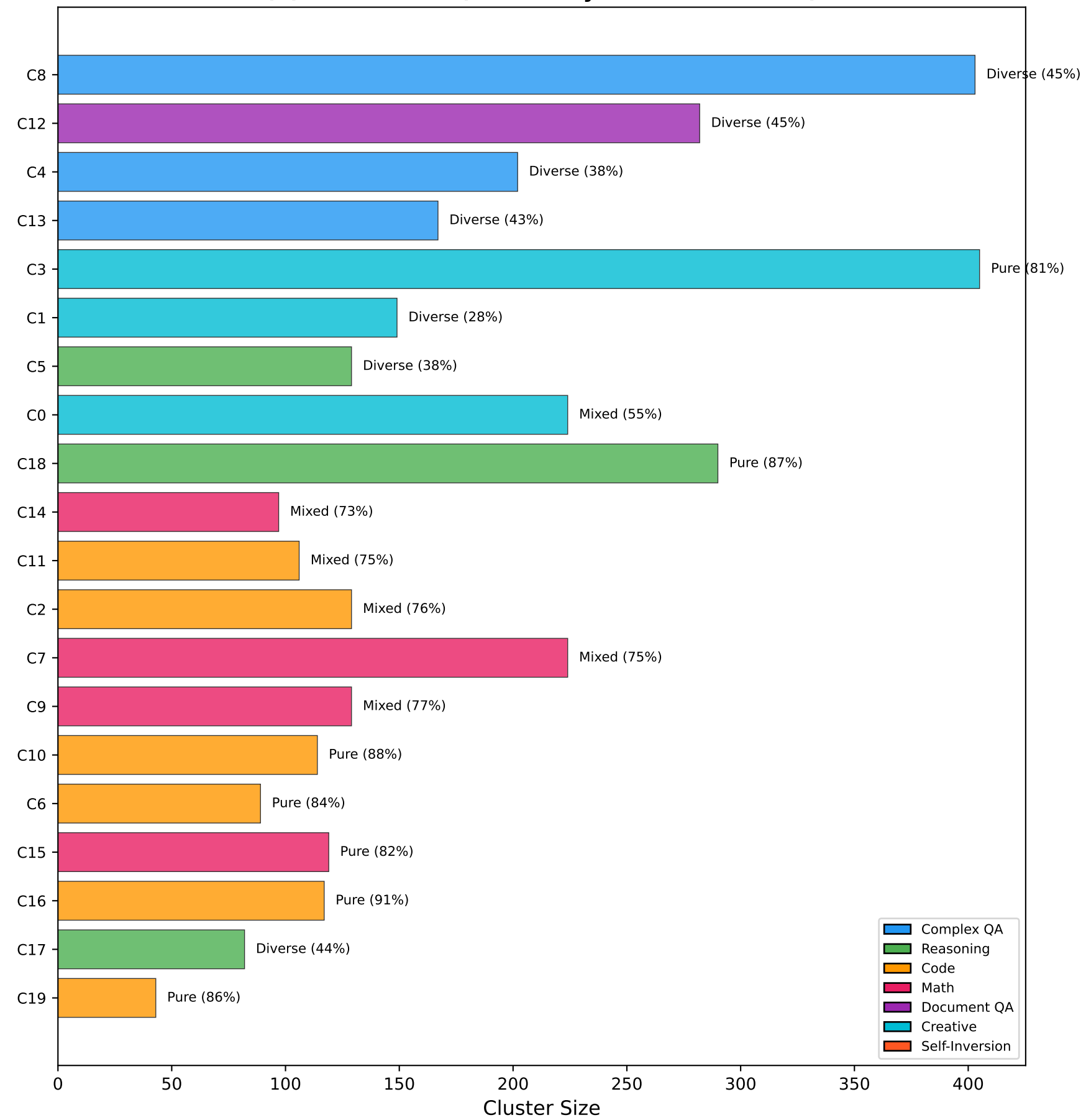
(b) Cluster Size (colored by dominant source)
