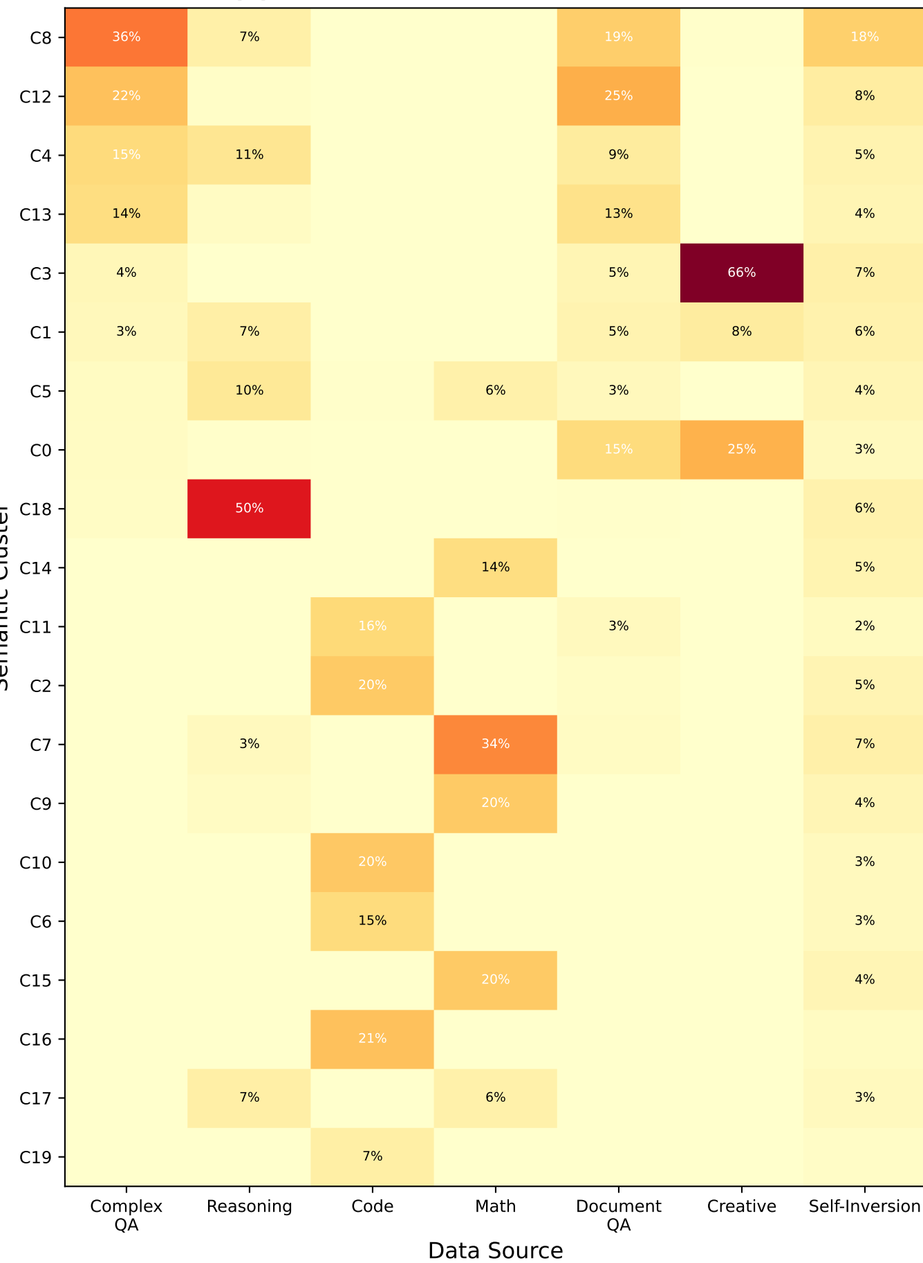
(a) Source Distribution Across Clusters
