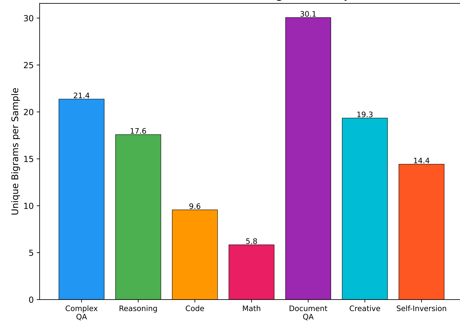
(c) Lexical Richness (Bigrams/Sample)
