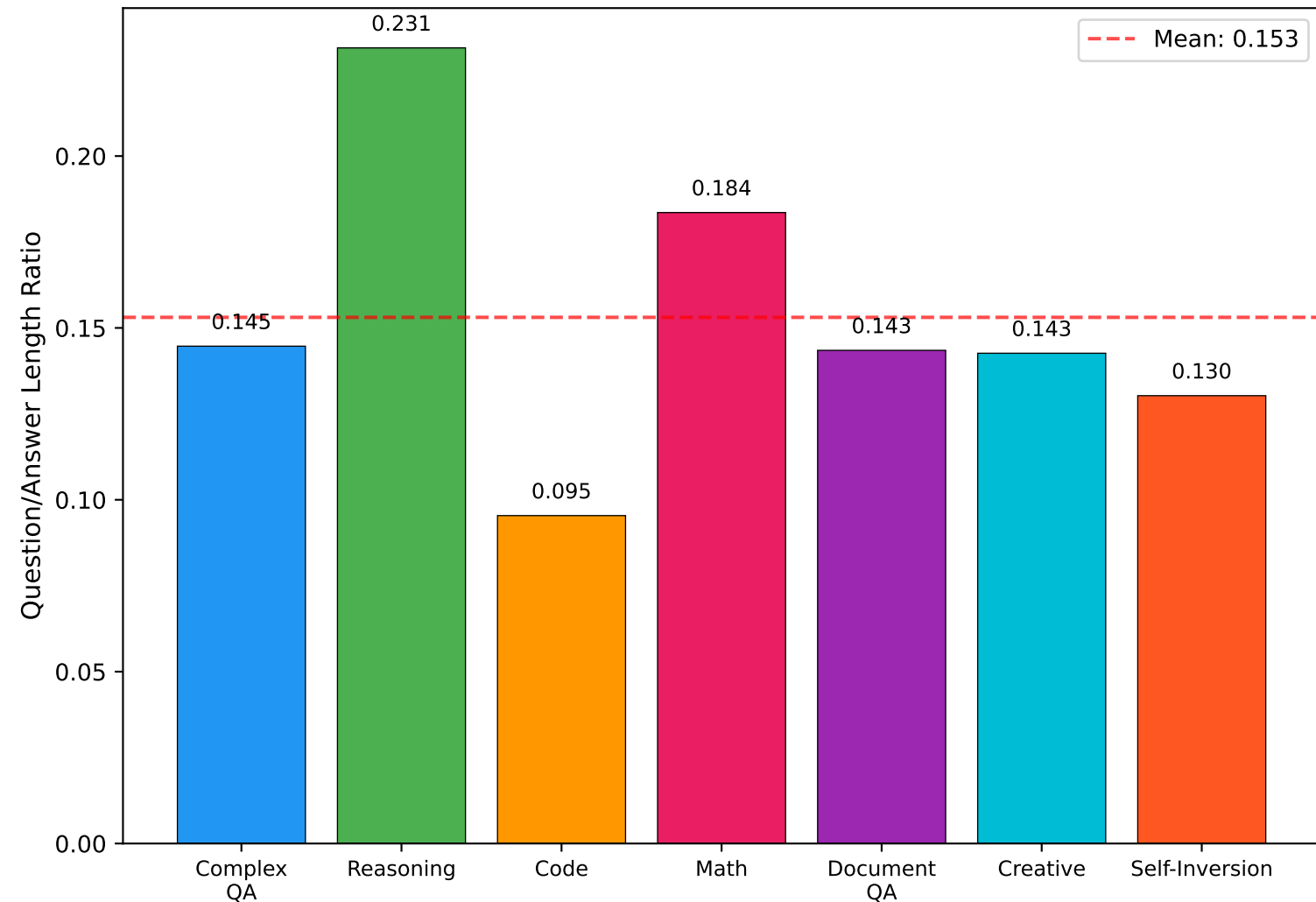
(b) Question Conciseness (Q/A Ratio)
