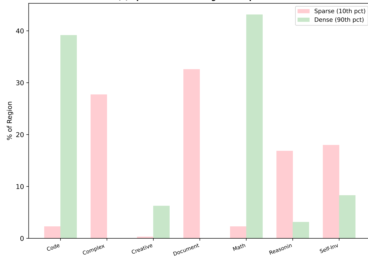
(c) Sparse vs Dense Region Composition
