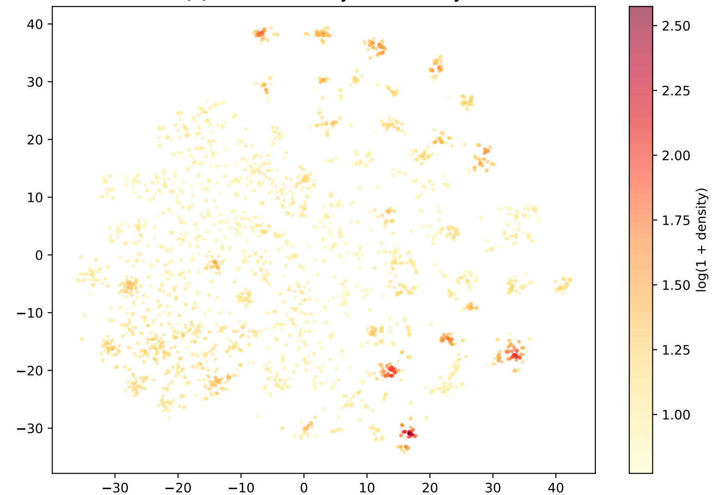
(b) t-SNE Colored by Local Density
