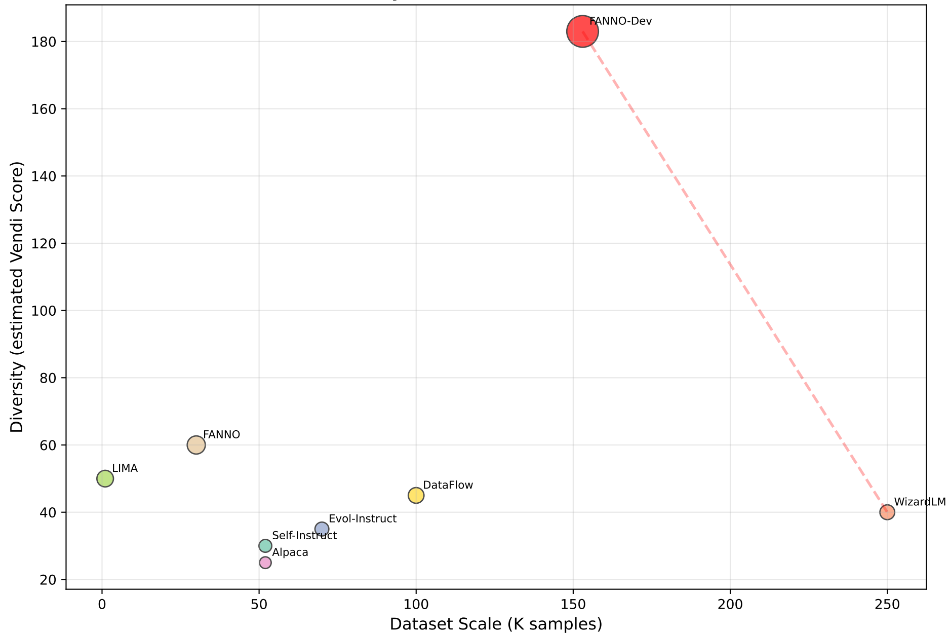
Scale vs Diversity: FANNO-Dev Dominates the Frontier
