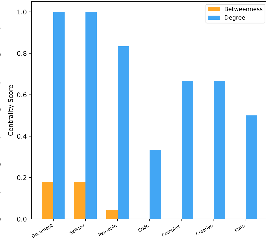
(c) Network Centrality Ranking
