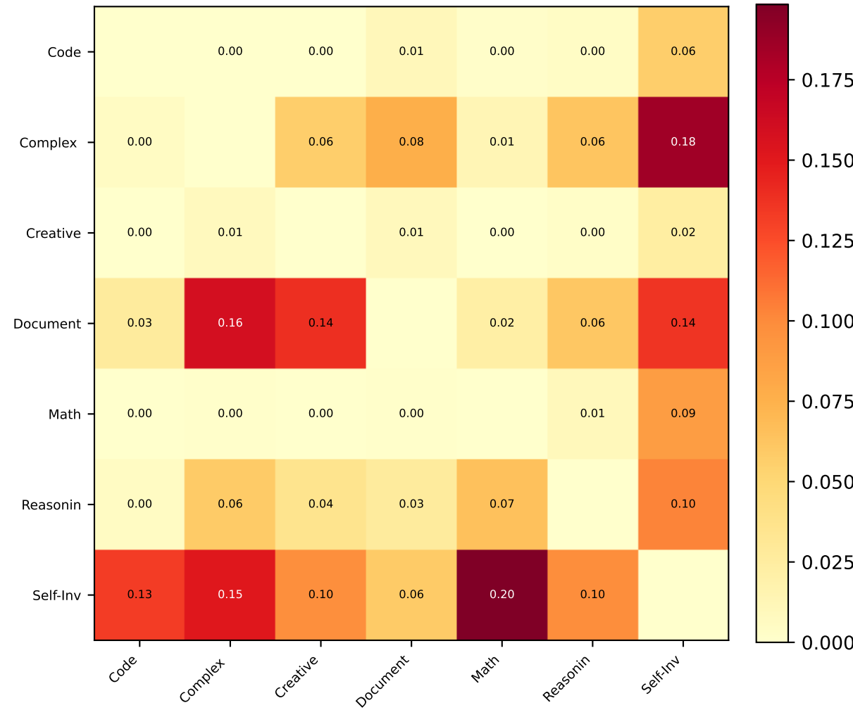
(b) Bidirectional KNN Overlap (K=20)
