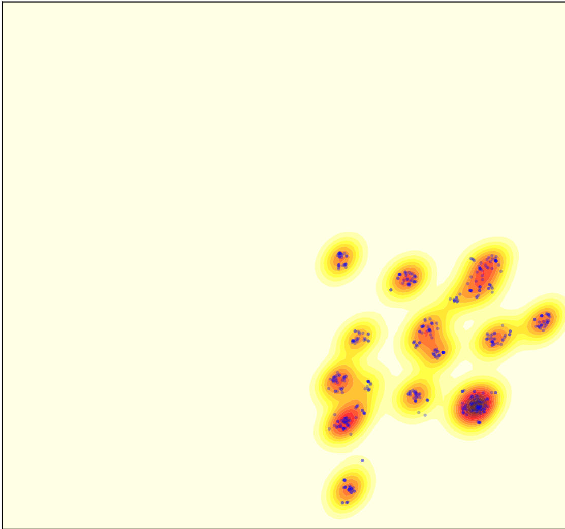
Math
