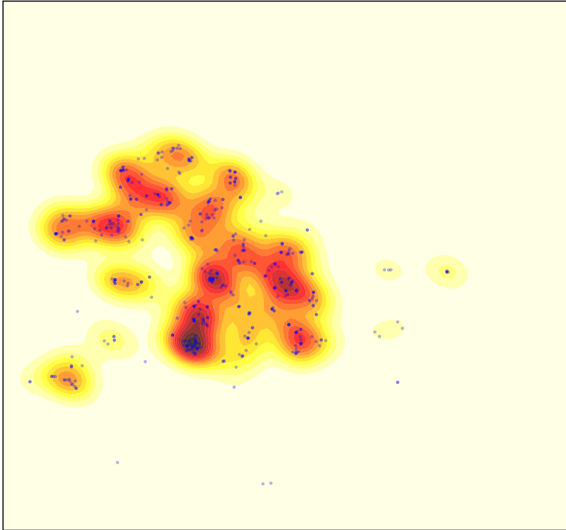
Reasoning
