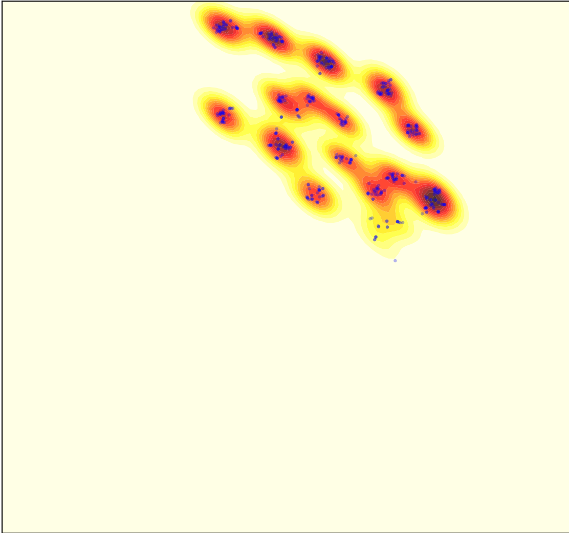
Math
