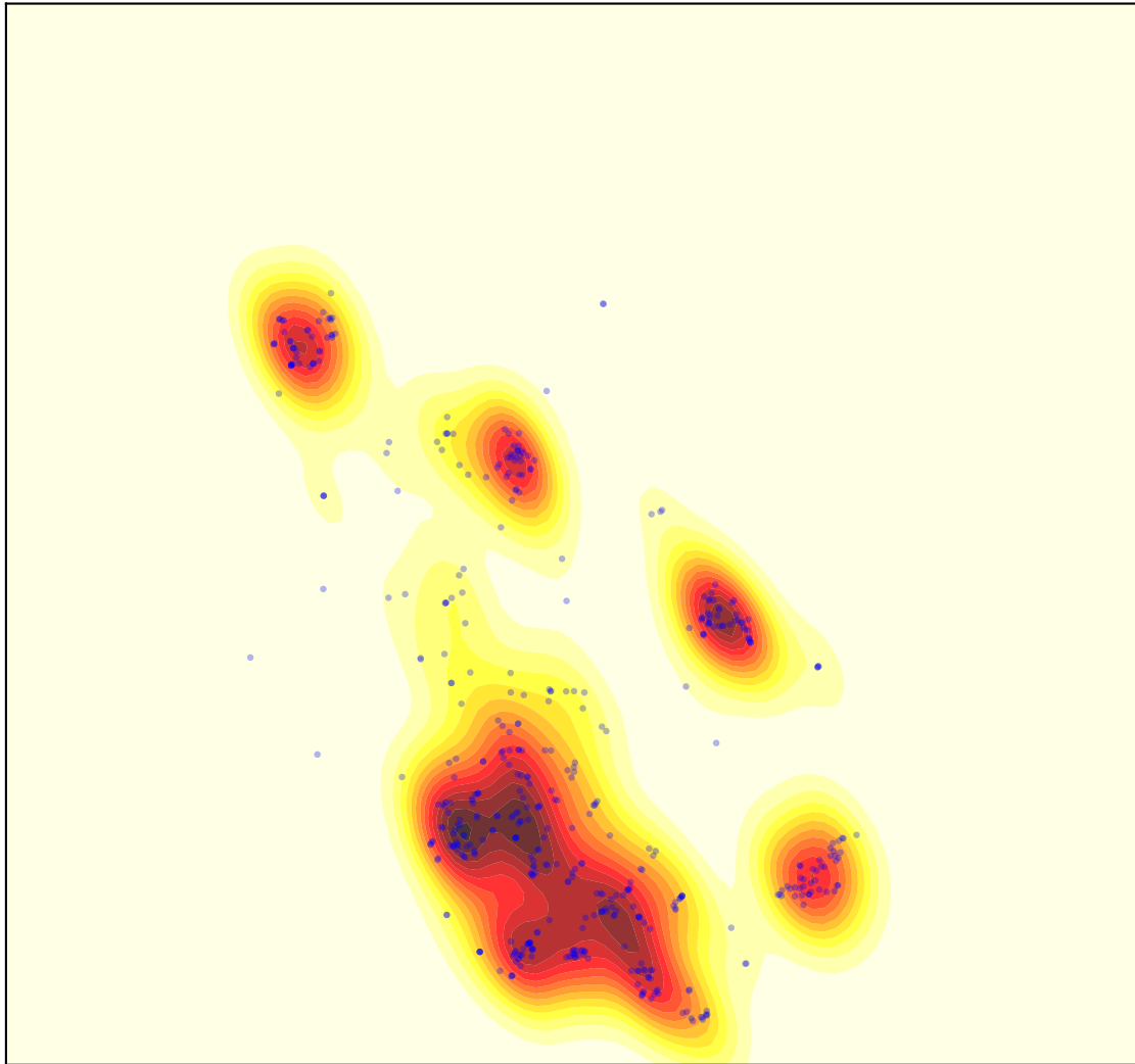
Reasoning
