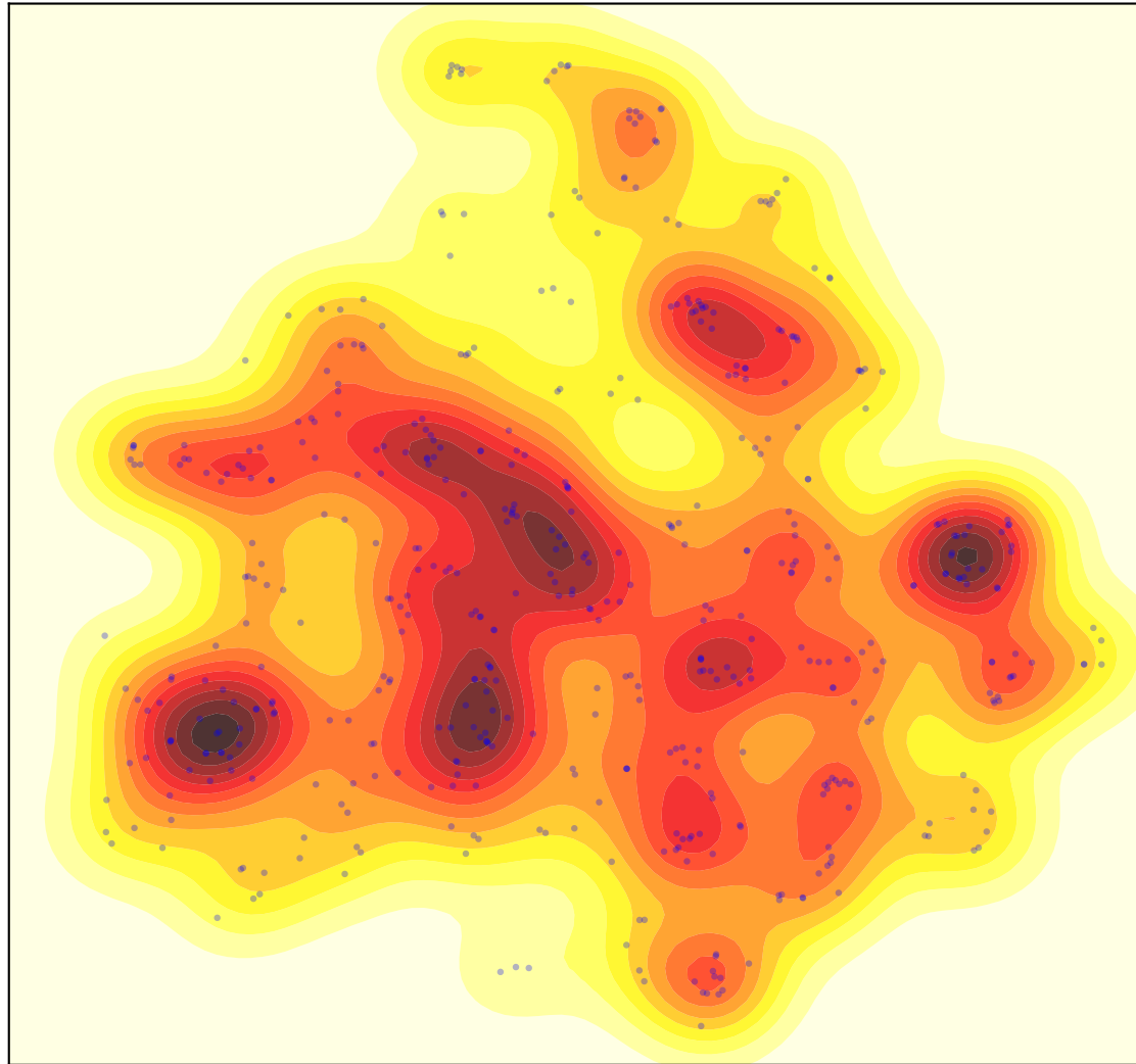
Self-Inversion
