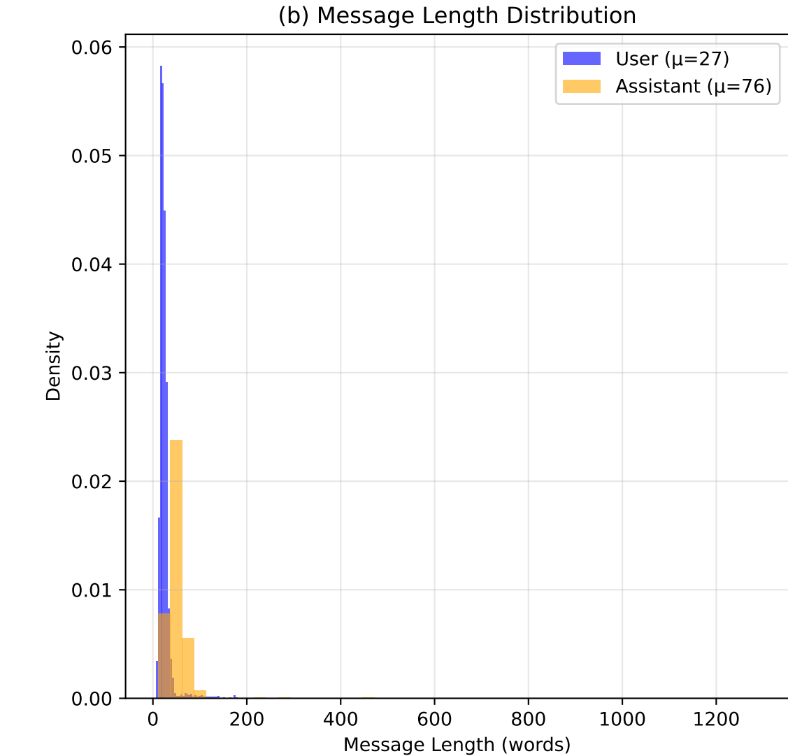
Fig 123: Multi-Turn Conversation Quality Deep Dive
