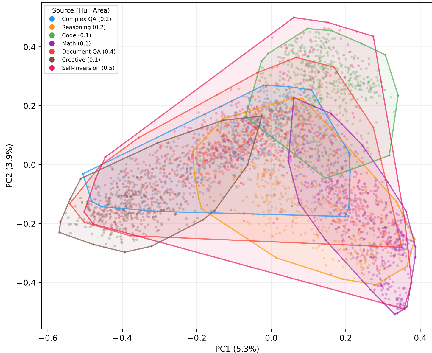
(a) Convex Hull Coverage (PCA 2D)
