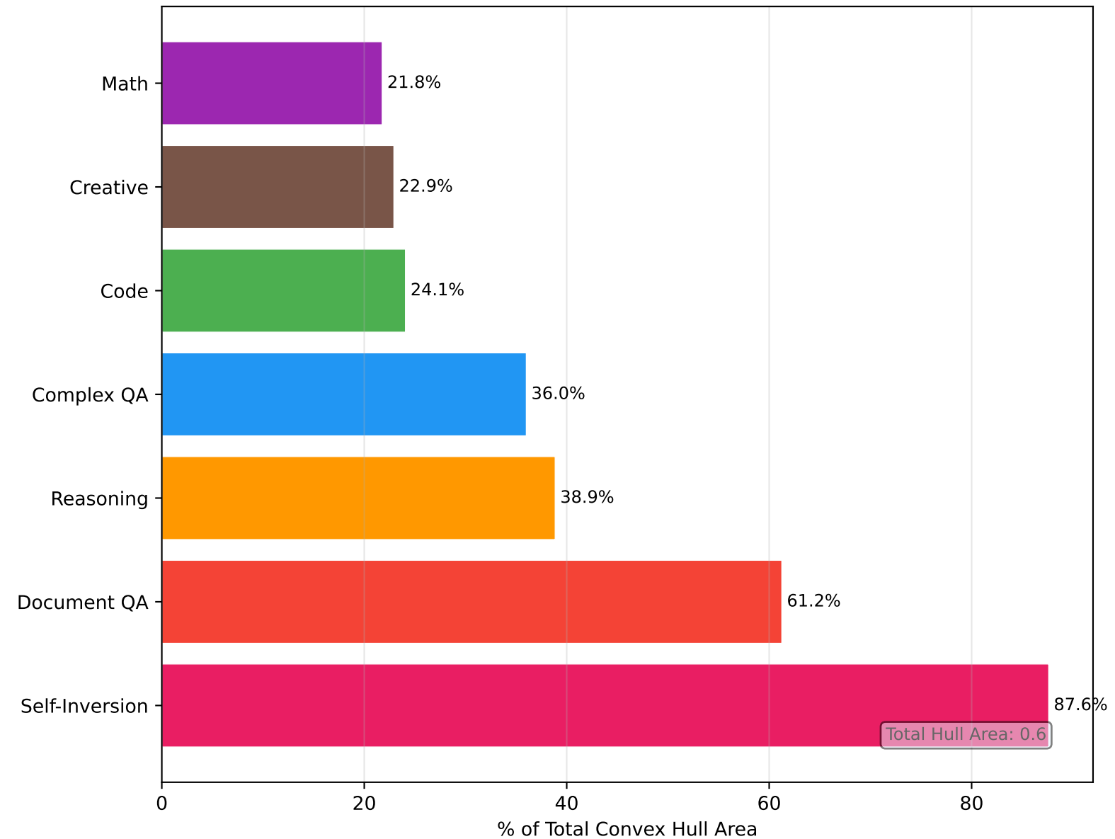
(b) Source Coverage (% of Total Area)
