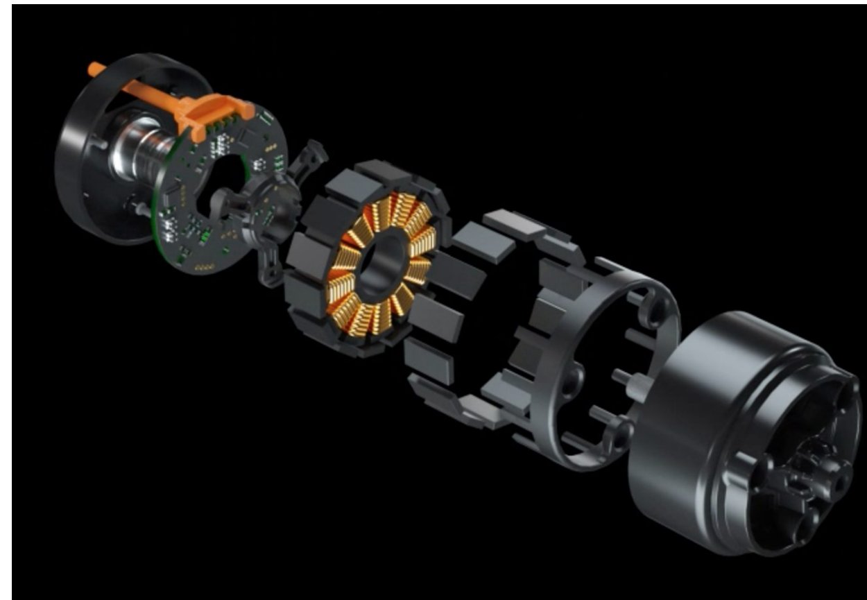
Infinite charging hub motor
