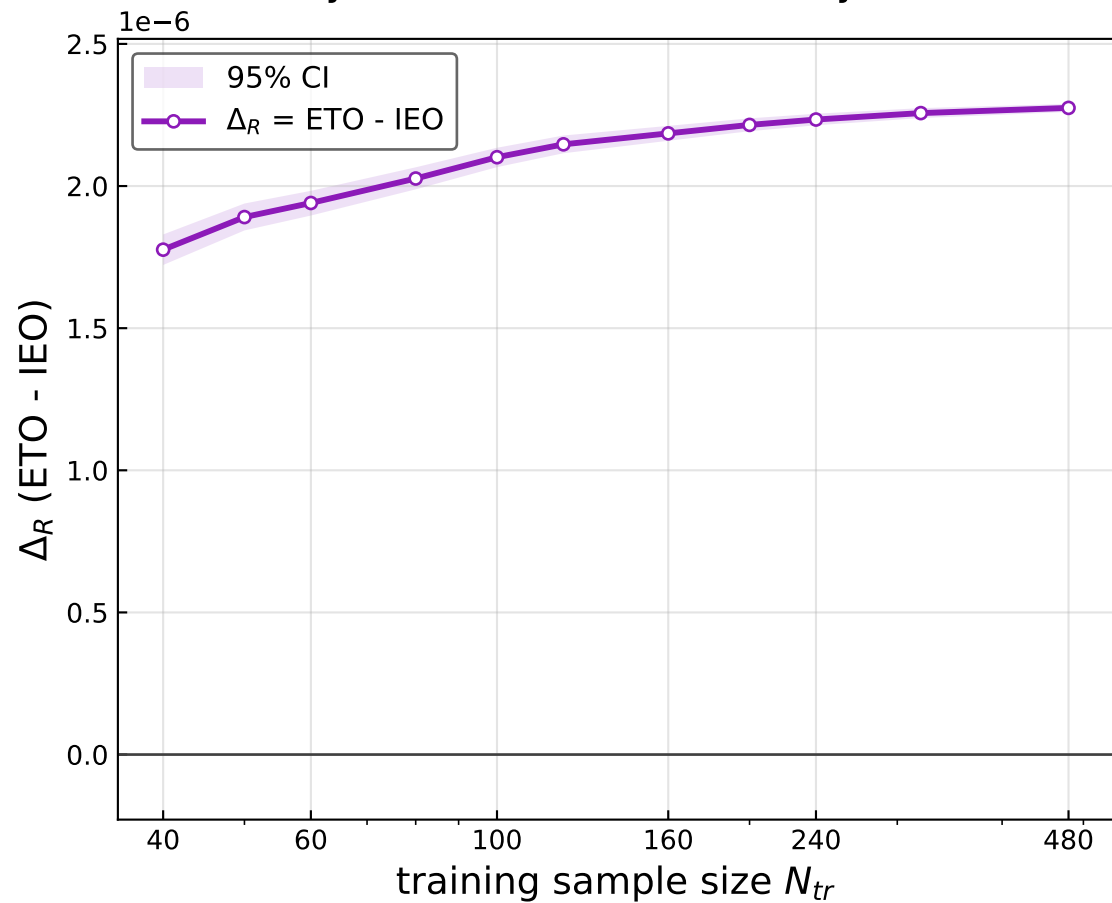
Severely ill-conditioned stationary Gaussian
