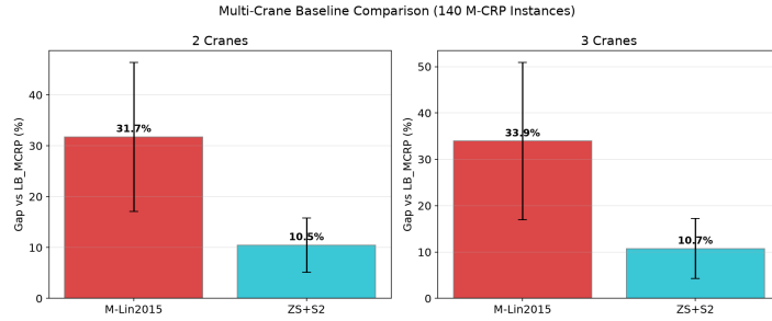
Figure 5: ZeroShot+S2 vs M-Lin2015 on 140 M-CRP instances. ZS+S2 achieves 10.46% ( C=2 ) and 10.74% ( C=3 ), outperforming M-Lin2015 (31.73% and 33.93%) by approximately 3\times .
